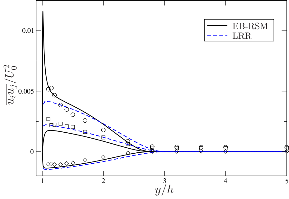
Figure 4: Reynolds stress profiles at the inlet ( x/h = -4 ). Comparison between models and experiment [9]. \circ \overline{u^2} , \square \overline{v^2} , \diamond \overline{uv} .
