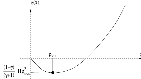
Figure 3: Function g : the minimum is attained at point \rho_{son} .
