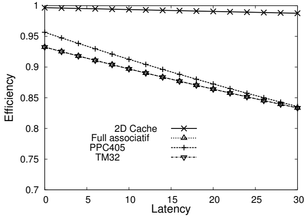
(a) 2D Backprojection: cache size=0.5 KB
