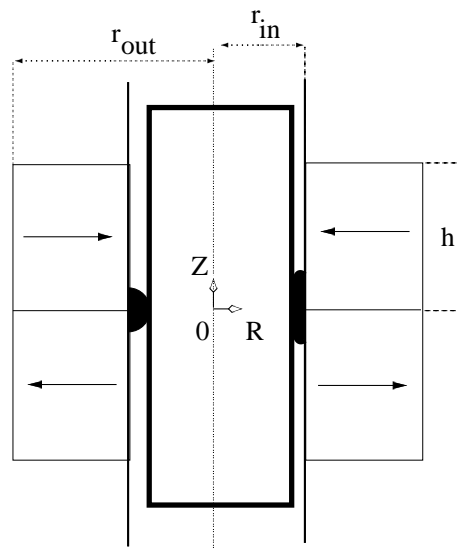
Figure 11. Radially moved away cylinder, crushed ferrofluid
