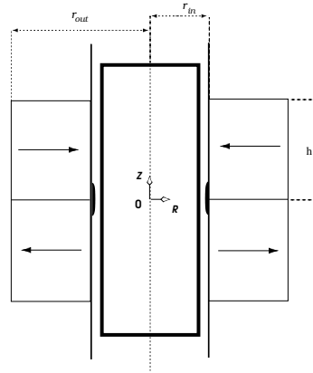
Figure 8. Geometry: two ring permanent magnets and an inner non-magnetic cylinder; air gap in the seal
