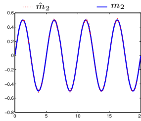
Fig. 10. Fault m_2 and its estimate \hat{m}_2 by (27)
