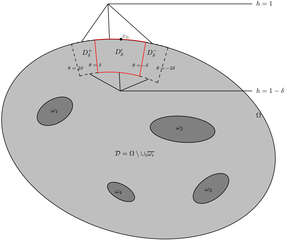
Figure 1: Decomposition of \mathcal{D}
