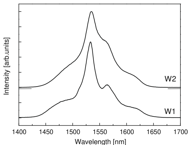
Fig. 6. Room temperature luminescence spectra of the ^4\text{I}_{13/2} \rightarrow ^4\text{I}_{15/2} transition of \text{Er}^{3+} ion for the W1, W2 planar waveguides, obtained by exciting the \text{TE}_{00} mode at 514.5 nm.
