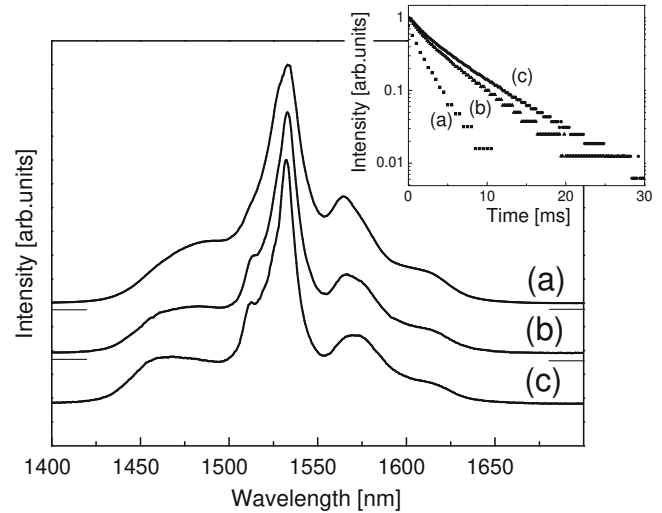
Fig. 4. Room temperature luminescence spectra of the 4 I 13/2 → 4 I 15/2 transition of Er 3+ ion for the (a) W900, (b) W1000, (c) W1100 planar waveguides, obtained by exciting the TE 0 mode at 514.5 nm. In the inset are reported the decay curves of the luminescence from the 4 I 13/2 → 4 I 15/2 metastable state of Er 3+ ions for the respective samples upon 514.5 nm excitation [18,19].
