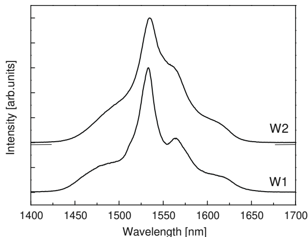
Fig. 6. Room temperature luminescence spectra of the {}^4\text{I}_{13/2} \rightarrow {}^4\text{I}_{15/2} transition of \text{Er}^{3+} ion for the W1, W2 planar waveguides, obtained by exciting the \text{TE}_{00} mode at 514.5 nm.
