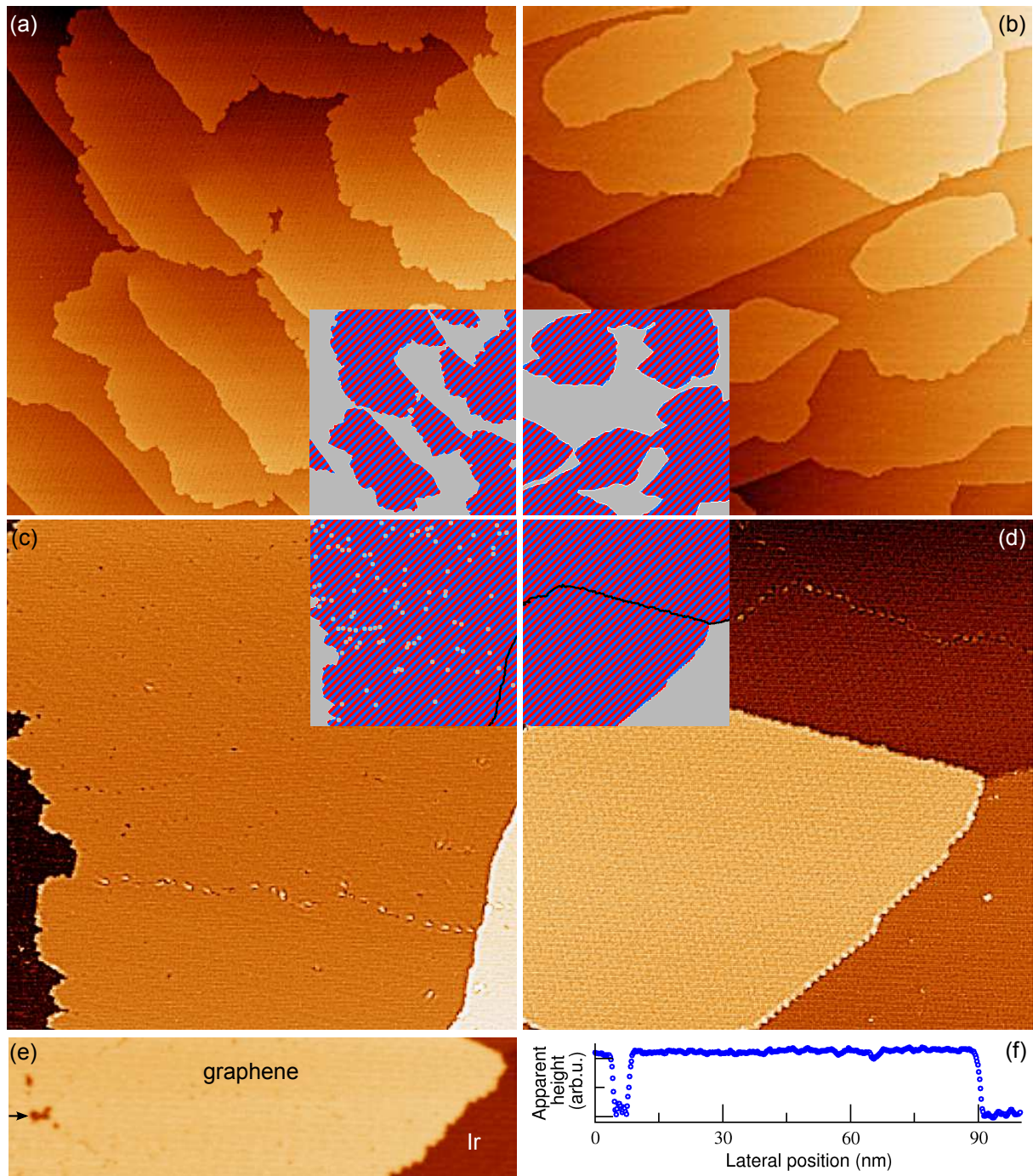
Figure 9. STM topograph of graphene grown by CVD on a Ir(111) surface at 1120 K, with an ethene partial pressure of 5 \times 10^{-10} mbar, during 80 s, before (a,c) and after (b,d) annealing for 40 s to 1220 K. Image size is 500 nm \times 500 nm for (a,b) and 125 nm \times 125 nm for (c,d). Insets show the graphene (hashed areas) on top of Ir(111) (gray). Inset of (c) highlights holes (gray spots) in graphene, insets of (c) and (d) highlight the Ir step edge (black line). (e) STM topograph (102 nm \times 28 nm) of graphene grown by CVD on a Ir(111) surface at 1120 K, out of exposure to an ethene partial pressure of 4 \times 10^{-9} mbar, during 20 s, and (f) apparent height profile along the horizontal passing through the arrow in (e).
