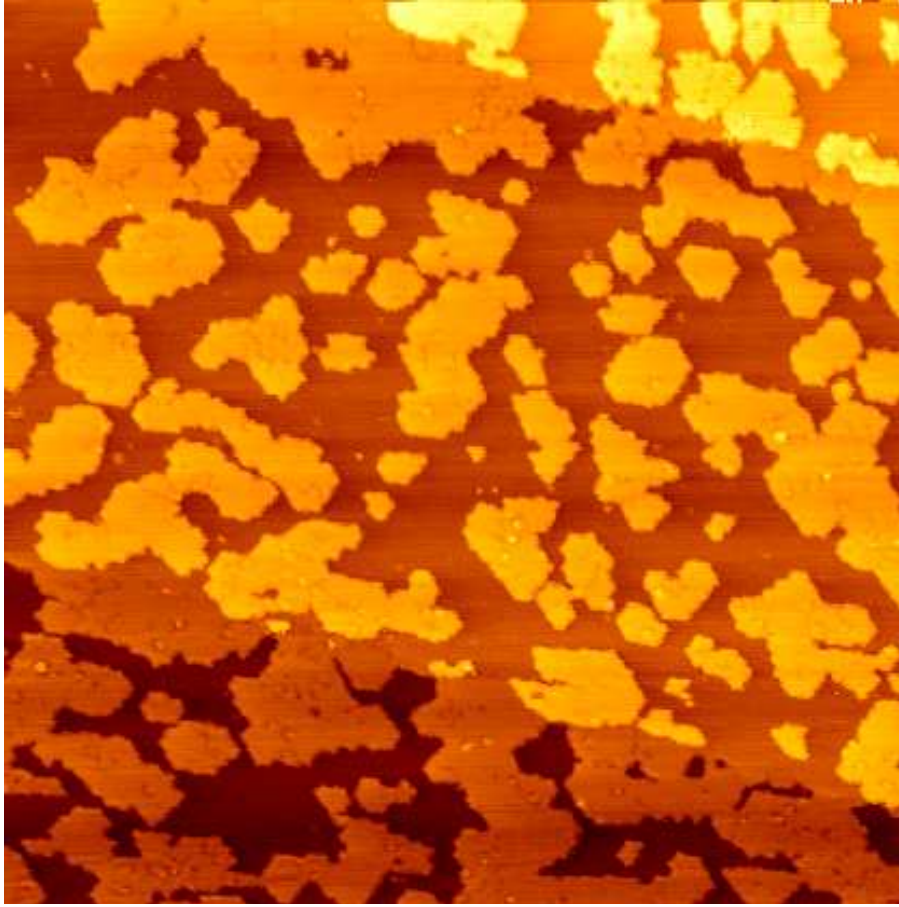
Figure 5. STM topograph (125 nm \times 125 nm, imaged at 300 K) of graphene prepared by TPG at 1120 K. 1.3 ML of coronene adsorbed at 125 K was used as molecular starting layer.
