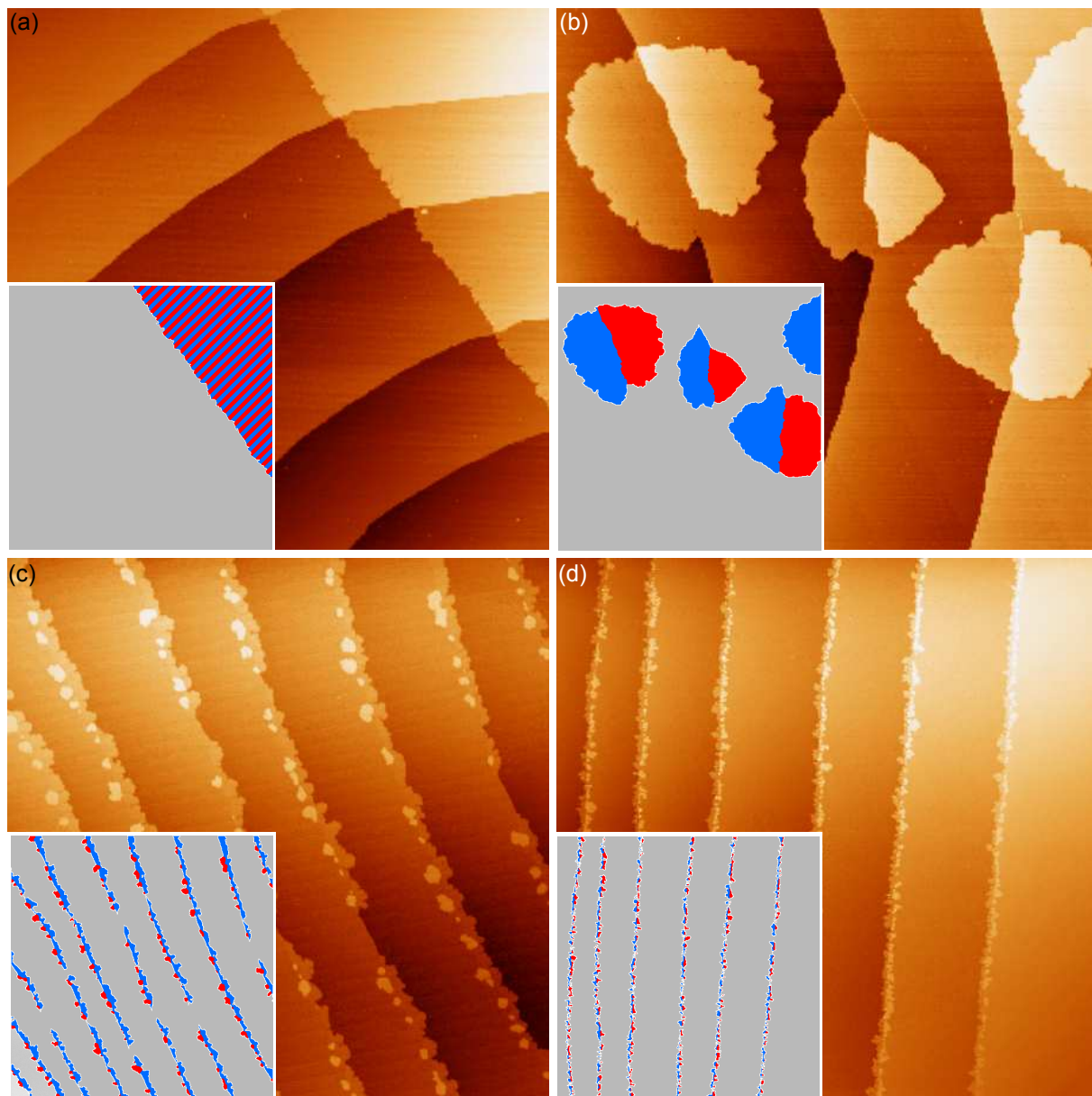
Figure 10. STM topograph ( 455 \text{ nm} \times 455 \text{ nm} ) of graphene grown by CVD on a Ir(111) surface at 1320 K (a), 1120 K (b), 970 K (c), and 870 K (d). The ethene partial pressure used for the growth of graphene is 5 \times 10^{-10} mbar, and the exposure time is 40 s, except for (a) where it is 80 s. Insets show graphene as hashed areas or in red (blue) when attached at a descending (ascending) step edge.
