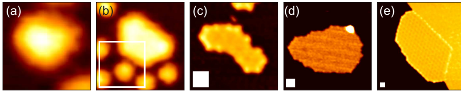
Figure 2. STM topographs of typical graphene islands prepared with the TPG procedure, after annealing for 20 s to (a) 870 K, 3.2 \text{ nm} \times 3.2 \text{ nm} , (b) 970 K, 6.2 \times 6.2 \text{ nm} , (c) 1120 K, 18 \text{ nm} \times 18 \text{ nm} , (d) 1320 K 32 \text{ nm} \times 32 \text{ nm} , (e) 1470 K, 64 \text{ nm} \times 64 \text{ nm} . The size of the white box corresponds to the size of the smallest topograph ( 3.2 \text{ nm} \times 3.2 \text{ nm} ). The islands undergo a transition from an undefined, probably amorphous state over a compact shape at low temperature to noncompact shapes at intermediate temperature (c) back to more compact shapes at high temperature.
