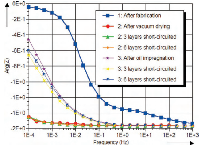
Figure 14. Frequency scans of the argument of the impedance, Z, for normal and short-circuited bushing layers following the three processing steps.
