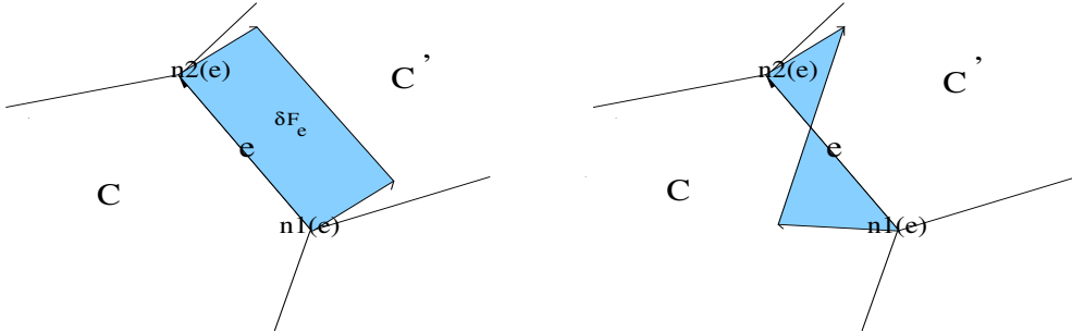
Figure 18. First order flux based on area swept by edge displacement \delta F_e of Margolin-Shashkov flux: donor cell interpretation (only one swept region at most)
