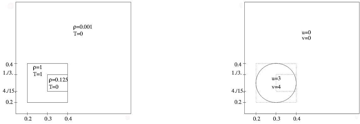
Figure 21. Initial data for test cases Planar geometry (density \rho and temperature T on Left, velocity \mathbf{U}=(u,v) on Right)
