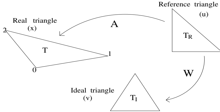
Figure 4. Different transformations between Real, Reference and Ideal triangle.
