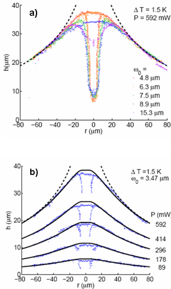
Figure 11 (adapted from Ref. [75]): Interface deformations when the laser shines upwards for (T - T_C) = 1.5 K . The dashed lines represent the pure buoyancy solution, when the Laplace pressure is ignored. a) Variation of the hump profile versus the beam waist \omega_0 . Away from the beam axis, all the profiles fall onto the same shape, demonstrating that only the laser power, and not \omega_0 , affects the large-scale hump shape. b) Calculated (solid line) and experimental (dots) hump profile for (T - T_C) = 1.5 K and \omega_0 = 4.8 \mu m .
