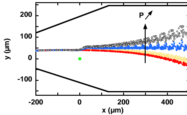
Figure 20 (adapted from Ref. [92]): Trajectory of the drop center of mass for various beam powers (from bottom to top: P = 0, 48, 53, 58 \text{ mW} ); switching occurs at P = 53 \text{ mW} . The beam location is indicated by the dot at (x=0, y=0) . Water flow rate Q_w = 0.05 \text{ } \mu\text{l}/\text{mn} , oil flow rate Q_o = 5 \text{ } \mu\text{l}/\text{mn} , U_o = 2.6 \text{ mm/s} , R = 60 \text{ } \mu\text{m} .
