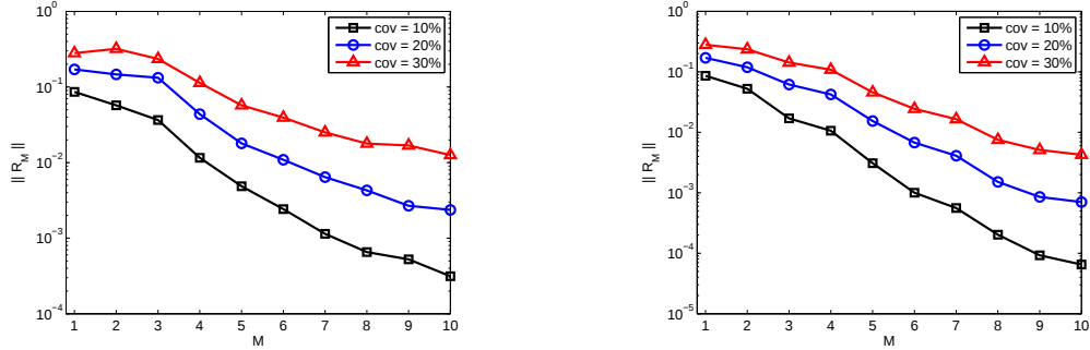
Figure 25. Impact of the input variability: convergence of algorithms 1 (left plot) and 2 (right plot), for different coefficients of variation (cov) of the four random variables, as indicated.
