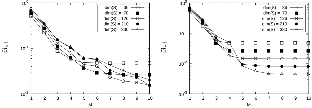
Figure 9. Convergence of the equation residual R_M with M for different dimensions of the stochastic space \mathcal{S} (corresponding to N_o = 3, \dots, 7 and fixed N = 4 ): algorithms 1 (left plot) and 2 (right plot).
