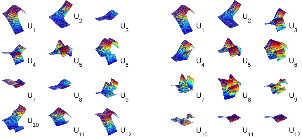
Figure 17. Comparison of the 12 first reduced modes with algorithms 1 (left plot) and 2 (right plot).
