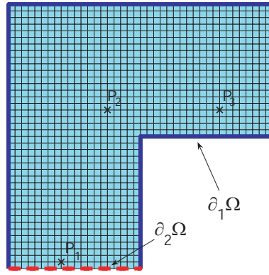
Fig. 1. Description of example 1: mesh and boundary conditions
