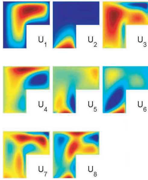
Fig. 16. Vectors \{U_i\}_{i=1}^8 obtained by (Direct-SD)
