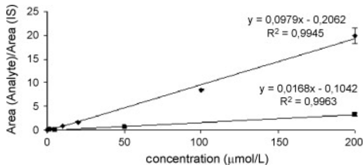
Fig. 1. D-Ribose-5-phosphate (■) and d-sedoheptulose-7-phosphate (◆) standard curves.
