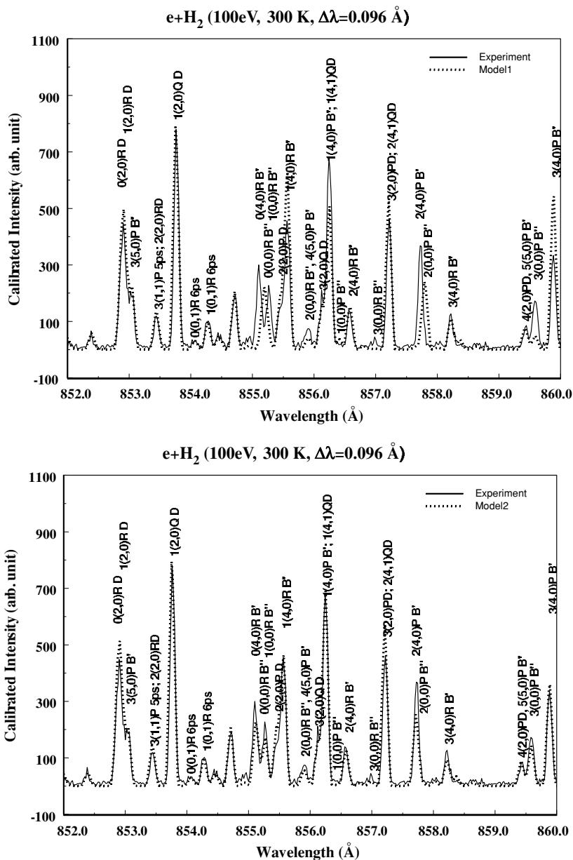
Figure 3. Comparison of observed (solid trace) and calculated (dot trace) spectra near the D' \ ^1\Pi_u(2) , B' \ ^1\Sigma_u^+(4) , and B'' \bar{B}' \ ^1\Sigma_u^+(0) - X \ ^1\Sigma_g^+(0) band transition region. The calculated spectrum (Model 1) in the top panel was calculated with the B' \ ^1\Sigma_u^+ - X \ ^1\Sigma_g^+ and D' \ ^1\Pi_u - X \ ^1\Sigma_g^+ transition probabilities of Abgrall et al. (1994) and adiabatic transition probabilities of the present work. Except for the partial B' \ ^1\Sigma_u^+ - D' \ ^1\Pi_u^+ interaction, nonadiabatic coupling among the B' \ ^1\Sigma_u^+ , D' \ ^1\Pi_u^+ , B'' \bar{B}' \ ^1\Sigma_u^+ , D' \ ^1\Pi_u^+ , and 5 p \sigma \ ^1\Sigma_u^+ states was neglected in the top panel. The dot trace in the bottom panel (Model 2) was obtained identically except for the use of the nonadiabatic transition probabilities for the B' \ ^1\Sigma_u^+ , D' \ ^1\Pi_u^+ , B'' \bar{B}' \ ^1\Sigma_u^+ , 5 p \sigma \ ^1\Sigma_u^+ , and D' \ ^1\Pi_u^+ - X \ ^1\Sigma_g^+ transitions. Transitions are labeled as J_i(v_j, v_i)\Delta J\beta , where i and j refer to the lower and upper states, \beta is electronic designation of singlet- ungerade states, and \Delta J = -1, 0 , and +1 correspond to P, Q , and R transitions, respectively.
