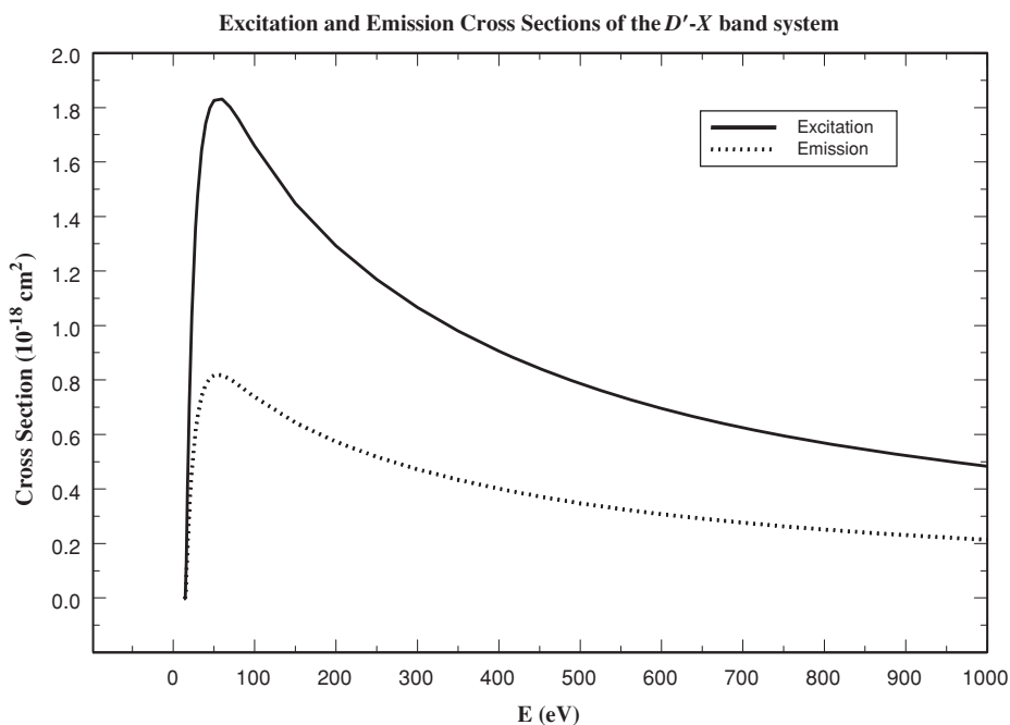
Figure 5. Excitation (solid) and emission (dotted) cross sections of the D'^1\Pi_u - X^1\Sigma_g^+ band system as a function of excitation energy at T = 300 K.
