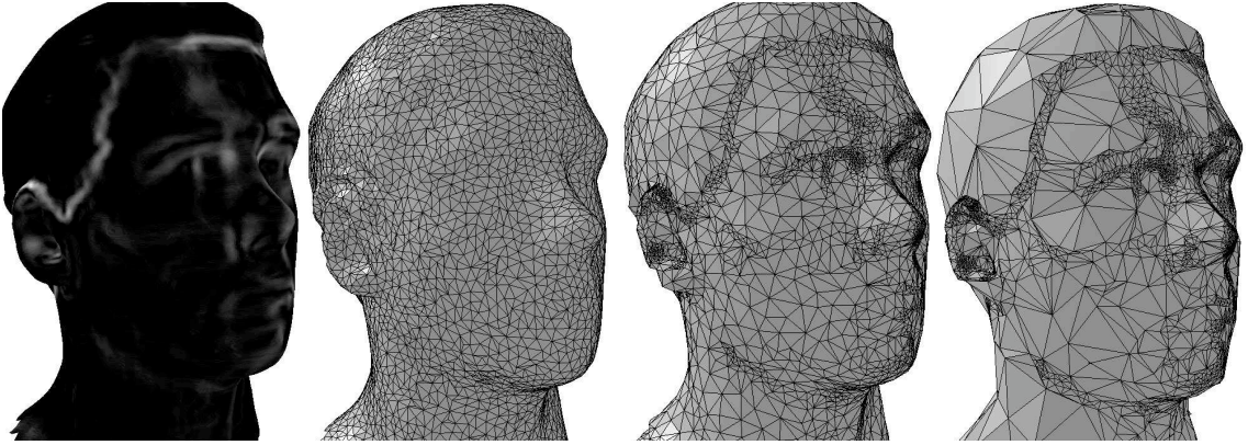
Figure 2.20: Adaptive remeshing with a density given by a texture.
