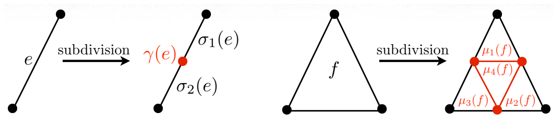
Figure 4.1: Edge-splitting subdivision.
