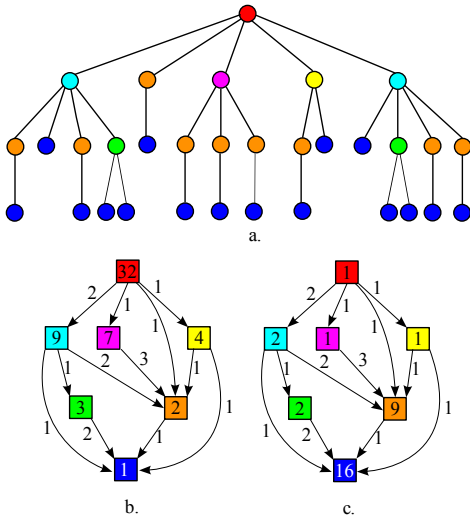
Fig. 2. a. A tree T whose vertices are colored according to their signature. b. Corresponding reduction graph showing the value with n(I) on each vertex. c. Reduction graph where vertices are valued with m(I) . Both quantities are computed recursively.
