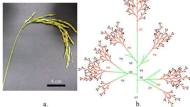
Fig. 18. a) photo of a rice panicle (courtesy of Y. Caraglio). b) corresponding topological structure (reconstructed with the AMAPmod/VPlants open software [62]).
