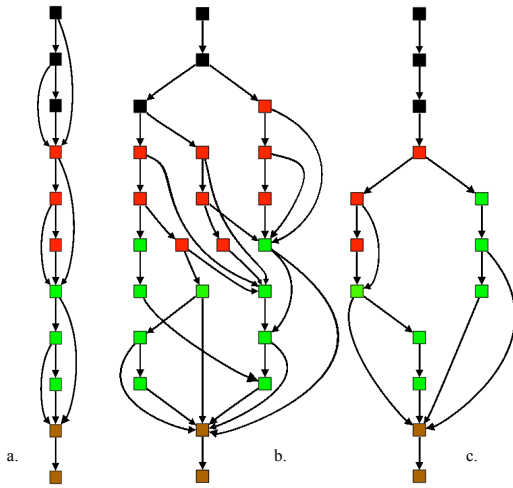
Fig. 12. DAGs corresponding to the reductions of tree individuals in the families a. T_0 , b. T_{0,4} and c. T_{0,8} .
