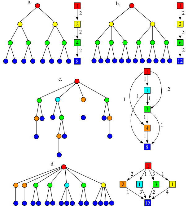
Fig. 4. Examples of a-c. different self-nested trees and their reduction graphs. d. a non-self-nested tree.
