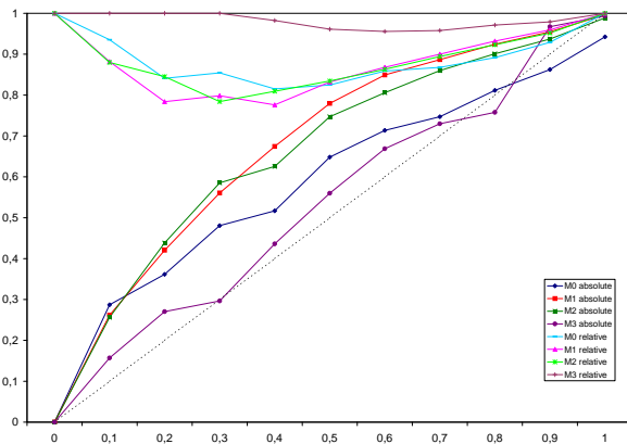
Fig. 13. Average vertex absolute and relative compression factors ( \rho_v(T) and \rho'_v(T) ) of the trees in the \mathcal{T}_i families, i = 0, 1, 2, 3 (standard deviations are not shown here). Abscissa represents branching probability. Curves passing through the point (0,0) correspond to the absolute coefficients.
