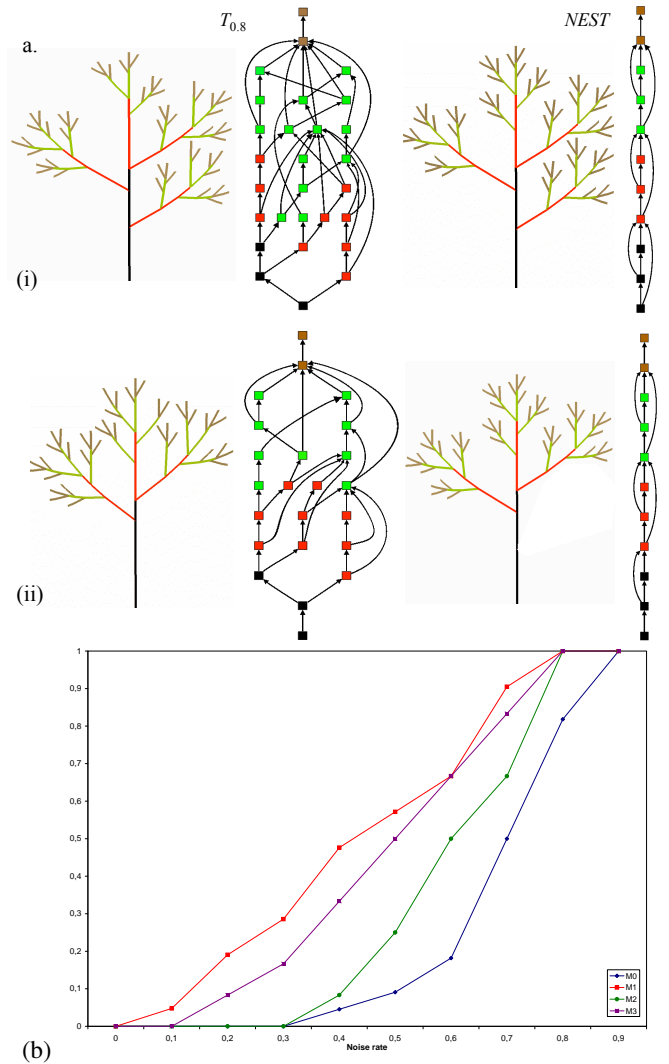
Fig. 17. a. Two random versions of T_{0,8} such that (i) the NEST is isomorphic to the template or (ii) not. b. Cumulated percentage of plants from the different families having a NEST isomorphic to their template plant as a function of noise.
