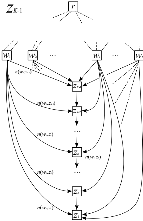
Fig. 6. DAG Z_{K-1} . The minimization D(Z_{K-1}, H) for H \in \mathcal{S}_K^+(Z_{K-1}) consists of merging all the vertices at level K in a minimal way to obtain a new DAG in \mathcal{S}_K^+(G) , i.e. linearized up to height K .
