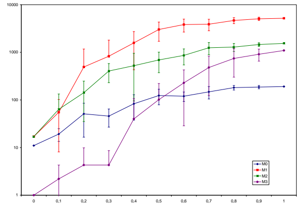
Fig. 15. Average number of vertices in \text{NEST}(T) for trees of the different families as a function of the branching probability.
