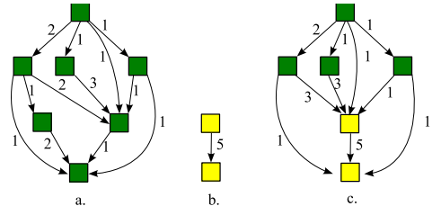
Fig. 5. a. a DAG G b. a linear DAG L such that h(L) \leq h(G) . c. DAG G \langle L \rangle corresponding to the DAG G partially linearized by L .
