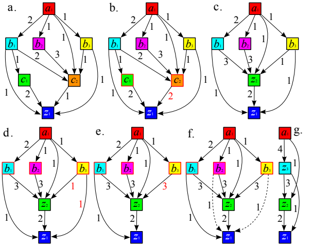
Fig. 7. The seven steps of the algorithm needed to find the nearest linear DAG of the DAG introduced in Fig. 2
