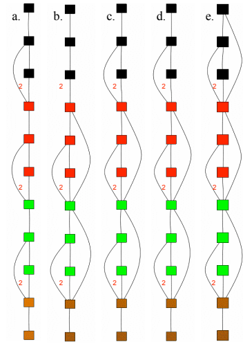
Fig. 14. \mathcal{R}(\text{NEST}(T)) corresponding to a. both T_0 and particular instances of b. T_{0,8} , c. T_{0,6} , d. T_{0,4} and e. T_{0,2} .
