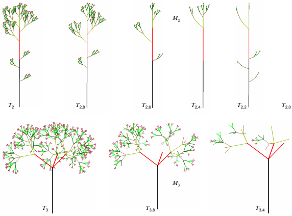
Fig. 11. Top row: template plant T_2 and trees in T_{2,i} for i = 8, 6, 4, 2, 0 . Bottom row: T_3 and 2 of its random versions from T_{3,8} , T_{3,4} .
