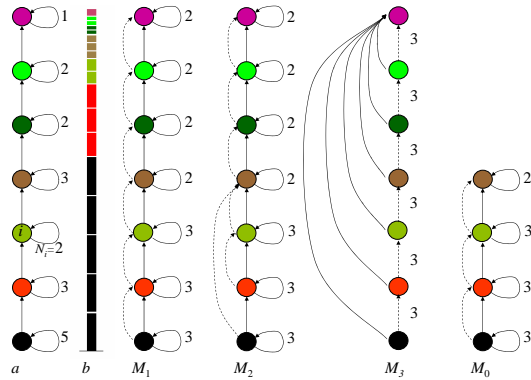
Fig. 8. Differentiation graphs used for the definition of theoretical plants. a) The differentiation graph of a non-branching plant structure. b) The resulting axis structure, where component colors correspond to the differentiation graph states in which these components were created. The numbers attached to each loop indicate the number of steps a meristem stays in the corresponding state. Right: The differentiation graphs of models M_1 , M_2 , M_3 and M_0 . Solid arrows correspond to possible transitions of the apical meristem states. Dashed arrows correspond to possible transitions from the apical meristem state to the axillary meristem states.
