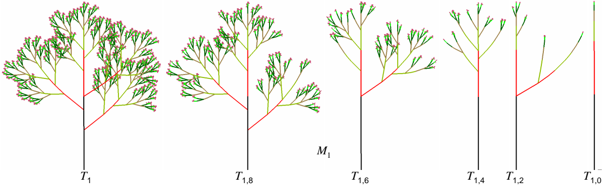
Fig. 9. Template plant T_1 corresponding to model and M_1 , and 5 of its random versions from the plant samples T_{1,8} , T_{1,6} , T_{1,4} , T_{1,2} , T_{1,0}
