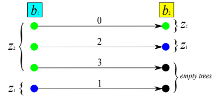
Fig. 22. Bipartite Matching problem associated with Fig. 7c.
