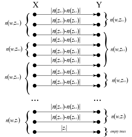
Fig. 21. Bipartite Matching Problem in the general case
