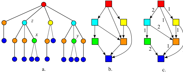
Fig. 1. a. A rooted tree T . Isomorphic nodes are colored identically: T[x] \equiv T[y] and z \preceq x then T[y] \sqsubseteq T[z] . b. Quotient graph \mathcal{Q}(T) associated with T : vertices of this graph are equivalence classes colored according to the color of the class of isomorphic vertices they represent in T . c. Reduction graph of T corresponding to \mathcal{Q}(T) whose edges are labeled with the signature distribution function n .
