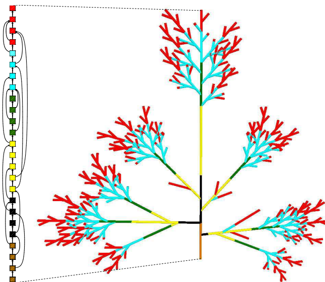
Fig. 20. a. An element T^* of NEST(T) b. Backward projection of the differentiation states inferred from T^* onto the initial tree structure of the panicle (see text for color interpretation).
