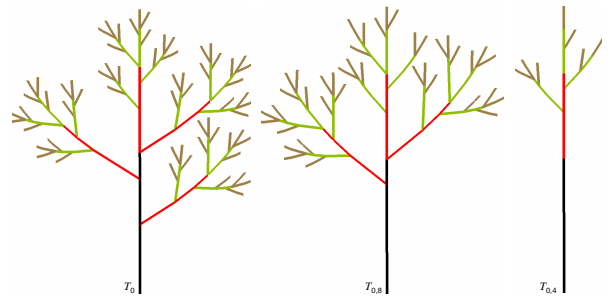
Fig. 10. The \mathcal{T}_0 family: (a) template plant T_0 and random trees from (b) \mathcal{T}_{0,8} and (c) \mathcal{T}_{0,4} .
