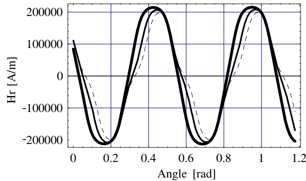
Figure 17. Representation of the radial field versus \theta produced by an optimized Halbach structure. r = 0.024 m, r_{\text{in}} = 0.025 m, r_{\text{out}} = 0.028 m, h = 0.003 m, J = 1 T, z = 0.0015 m, (thick line: the angular width ratio between the tile permanent magnets radially and tangentially magnetized is \frac{1}{3} ), (thin line: the ratio is \frac{3}{2} ), (dashed line: the ratio is 1).
