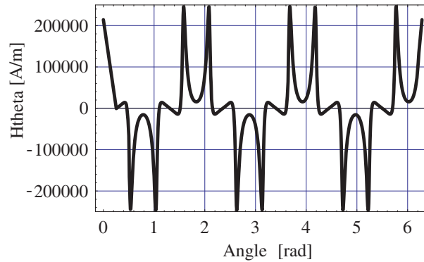
Figure 11. Azimuthal field created by a Halbach structure versus the angle \theta , the radial distance equals 0.5 mm from the magnets, r_{in} = 0.025 m, r_{out} = 0.028 m, h = 0.003 m, J = 1 T, z = 0.0015 m.
