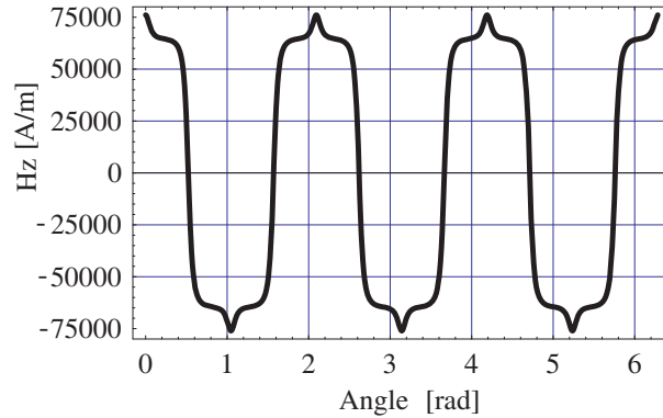
Figure 13. Axial field created by a Halbach structure versus the angle \theta , the radial distance equals 0.5mm from the magnets, r_{in} = 0.025 m, r_{out} = 0.028 m, h = 0.003 m, J = 1 T, z = 0.0015 m.
