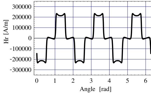
Figure 9. Radial field created by a Halbach structure versus the angle \theta , the radial distance equals 0.5 mm from the magnets, r_{in} = 0.025 m, r_{out} = 0.028 m, h = 0.003 m, J = 1 T, z = 0.0015 m.
