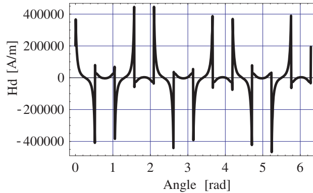
Figure 14. Representation of the azimuthal component of the demagnetizing field H_\theta inside the tile permanent magnets versus the angle \theta , the radial distance equals 0.2 mm from the inner faces of the tile permanent magnets, r_{in} = 0.025 m, r_{out} = 0.028 m, h = 0.003 m, J = 1 T, z = 0.0015 m.
