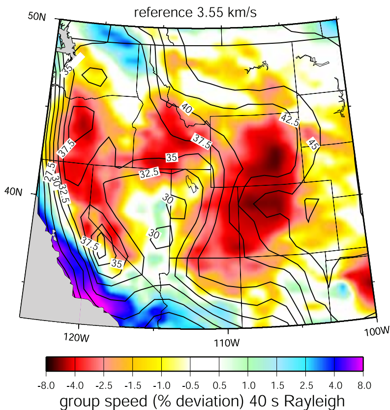
Figure 19. Rayleigh wave group speed dispersion map at 40 s period for the region outlined in Figure 14b. The Cornell US Moho depth model [Seber et al. , 1997] is plotted as contours with a 2.5 km contour interval with a maximum thickness (of 47 km) under Colorado. Low velocities generally correspond to thick crust.
