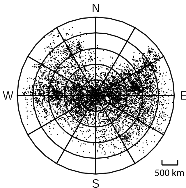
Figure 10. A plot of the azimuth and distance for all signals in the central-east region with SNR > 10 at 25 s period. The sparse regions in the N-NE and S-SW are due to the array configuration.
