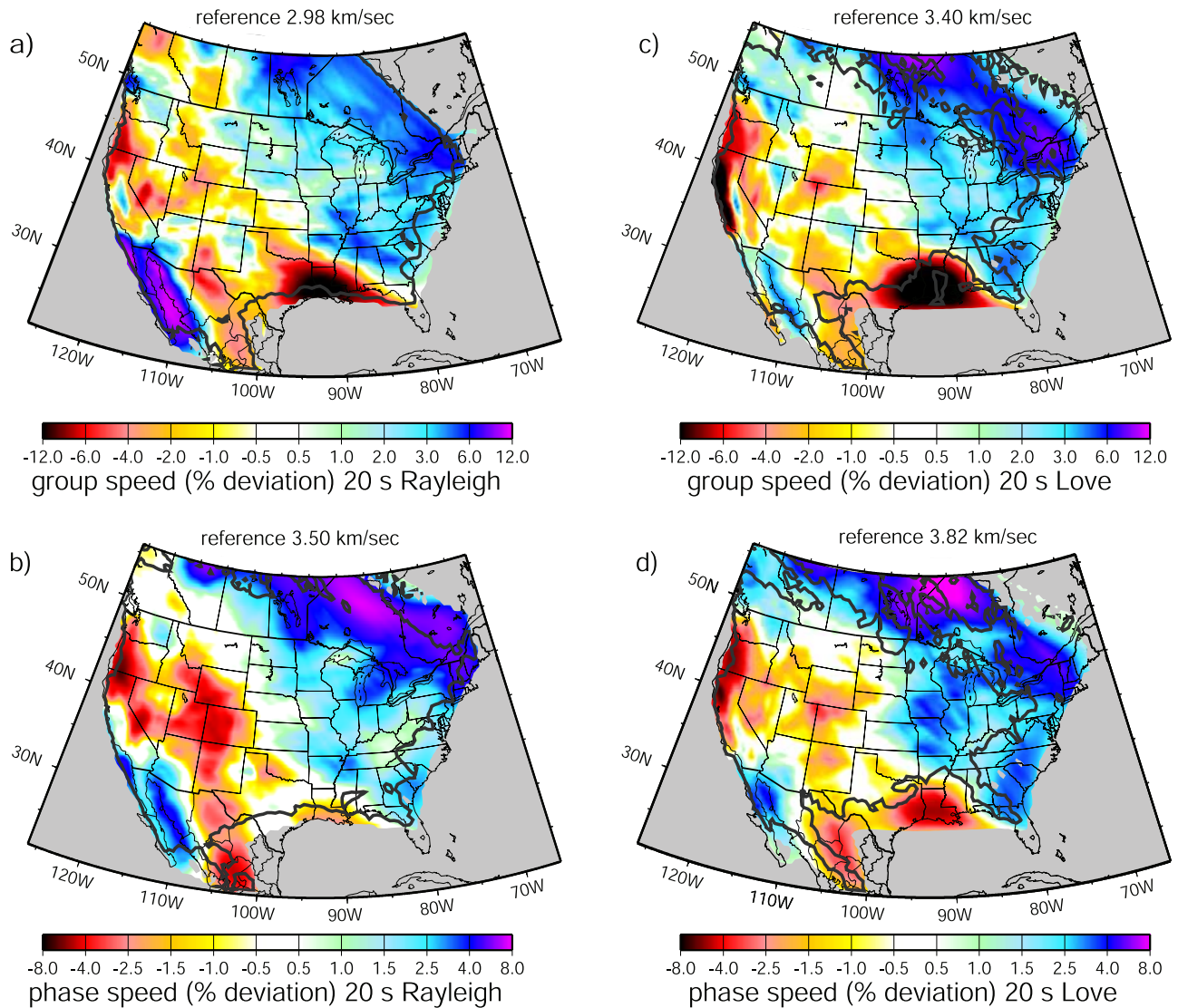
Figure 13. Same as Figure 12, but for 20 s period and sedimentary contours are suppressed.
