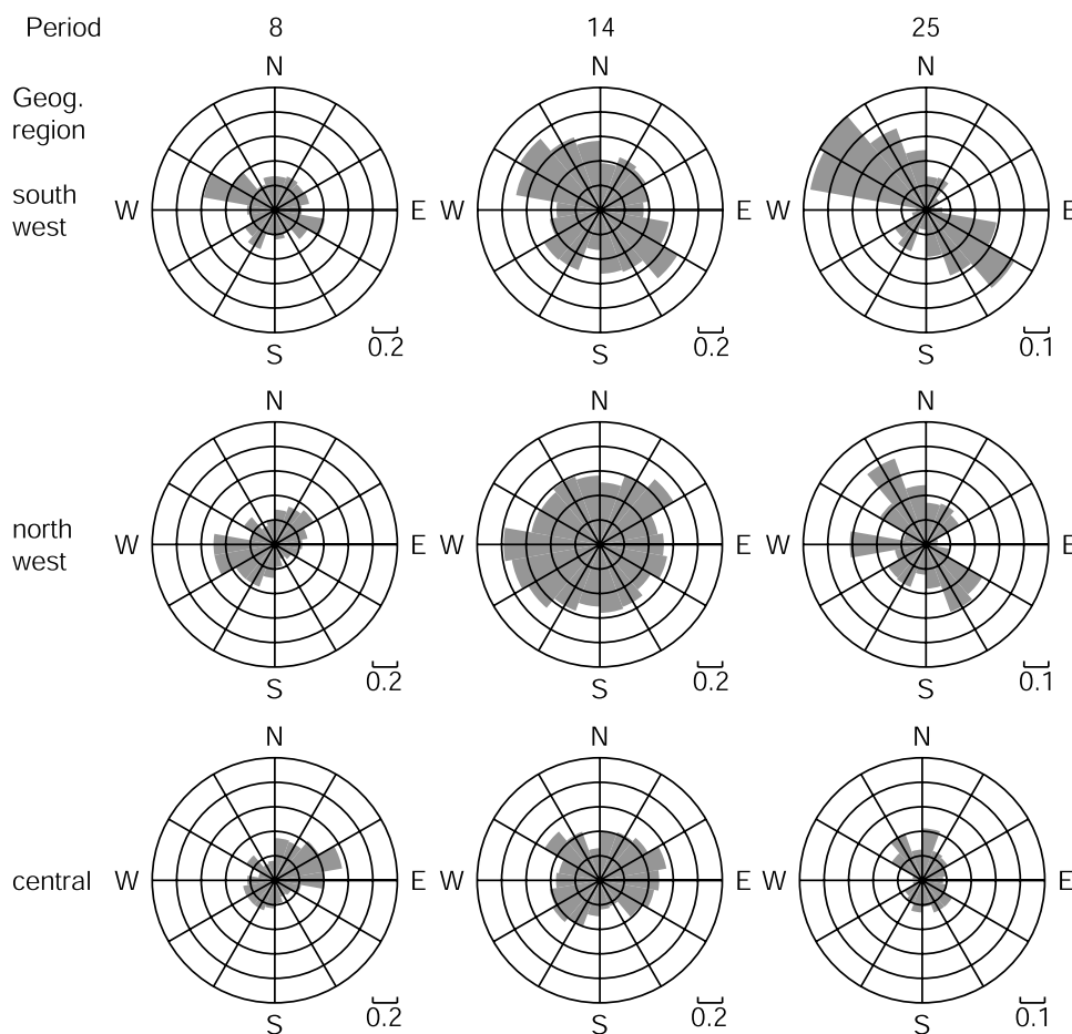
Figure 9. Same as Figure 8, but for Love waves.
