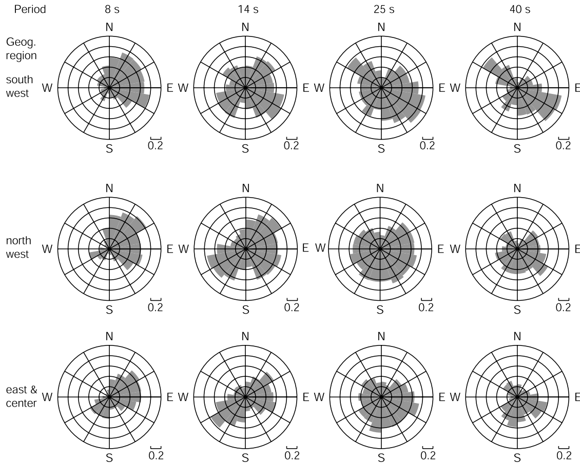
Figure 8. The directional dependence of high SNR (>10) Rayleigh wave EGF signals plotted at different periods (8, 14, 25, 40 s in different columns) and geographical sub-regions (different rows). Azimuth is the direction of propagation of the wave. Results are presented as fractions, in which the numerator is the number of inter-station paths in a particular azimuthal bin with SNR > 10 and the denominator is the number of paths in the bin (from Figure 1b).
