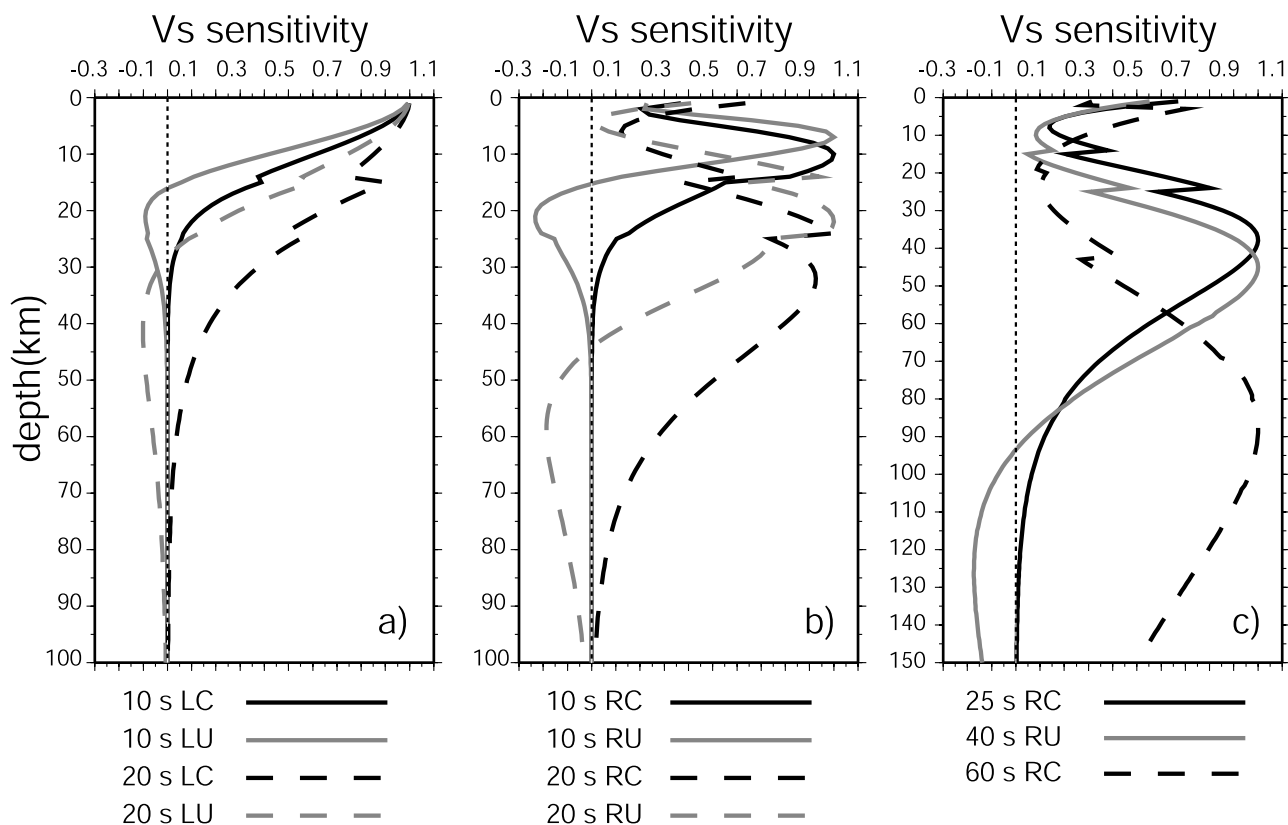
Figure 16. Sensitivity kernels for all dispersion maps shown here. Sensitivities for 10 and 20 s period Love waves are shown in Figure 16a, 10 and 20 s period Rayleigh waves are in Figure 16b and longer periods in Figure 16c. The kernels have been normalized to have the same maximum amplitude and the labeling is as follows: RC - Rayleigh phase, RU - Rayleigh group, LC - Love phase, LU - Love group. Kernels are computed for PREM but with the ocean replaced by consolidated sediments.
