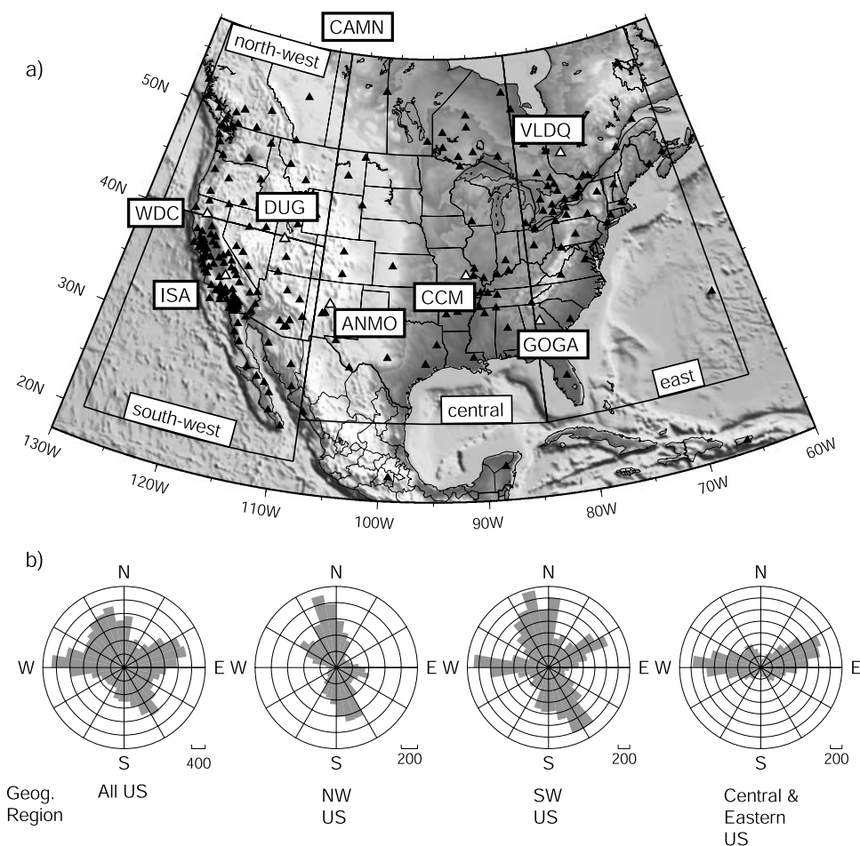
Figure 1. (a) The study area with stations represented as triangles. Larger white triangles with station names indicate inter-station paths for the waveforms and dispersion curves in Figure 2. The study area is divided into four boxed sub-regions. (b) Azimuthal distribution of inter-station paths, plotted as the number of paths per 10^\circ azimuthal bin, for the entire data set (at left) and in several sub-regions. Both azimuth and back-azimuth are included and indicate the direction of propagation of waves. Station CAMN is just north of the map boundary at 63.76, -110.89 .
