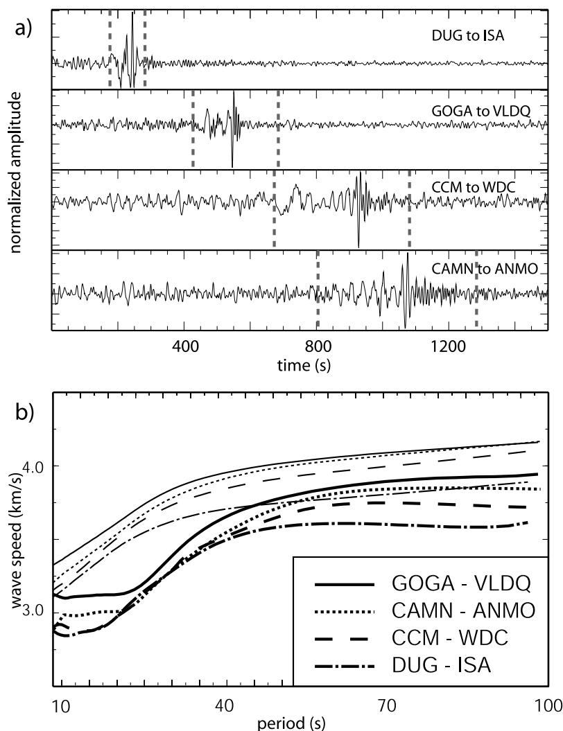
Figure 2. Examples of broadband vertical-component symmetric signal empirical Green functions (Rayleigh waves) through various tectonic regimes for the inter-station paths indicated with white triangles in Figure 1a. Waveforms are filtered between 7 and 100 s period. The time windows marked with vertical dashed lines are at 2.5 and 4.0 km/s. (b) The corresponding measured group and phase speed curves. Group velocity curves are thicker than phase velocity curves.
