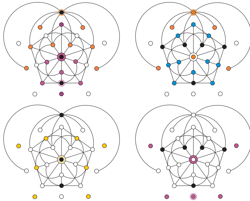
Figure 1: A pictorial illustration of the structure of the Veldkamp lines of \mathcal{V}(GQ(2,4)) . Left: – A line of Type I, comprising three distinct perps (distinguished by three different colours) having collinear centers (encircled). Right: – A line of Type II, featuring two perps with non-collinear centers (orange and purple) and a doily (blue). In both the cases the black bullets represent the common elements of the three hyperplanes.
