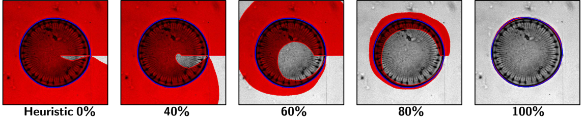
Figure 9: Globally optimal circular path extraction with increasing heuristic.
