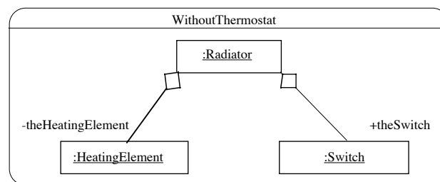
Figure 4 : Configuration diagram associated with the WithoutThermostat configuration-state
