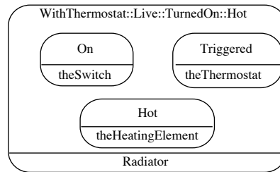
Figure 5 : Specification of the state WithThermostat::Live::TurnedOn::Hot of a Radiator composite object
