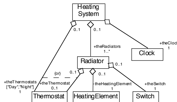
Figure 1 : Example of a composite class modeling heating systems
