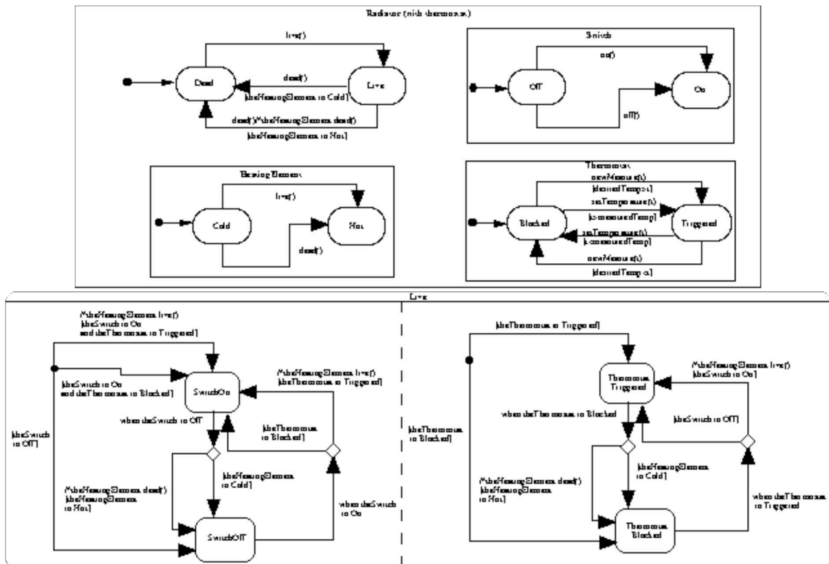
Figure 2 : Statechart diagram of the composite class Radiator
