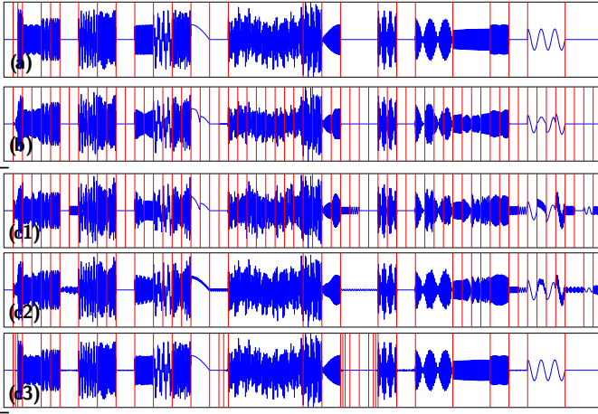
Fig. 3. (a) synthetic sound signal with 30 random cosine atoms N = 4096 ; (b) recovery using a fixed cosine basis; (c1) first iteration of the best basis recovery algorithm, n = N/3 ; (c2) iteration s = 5 ; (c3) iteration s = 20 .
