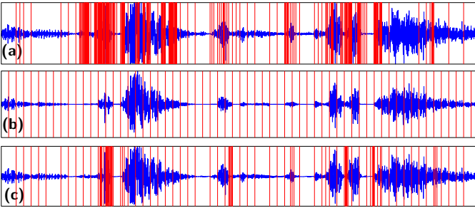
Fig. 4. (a) sound signal of a tiger howling, together with the best spatial segmentation, N = 32768 ; (b) recovery using fixed local cosine basis, n = N/3 (PSNR=19.24dB); (c) recovery using best cosine basis, n = N/3 (PSNR=21.32dB)
