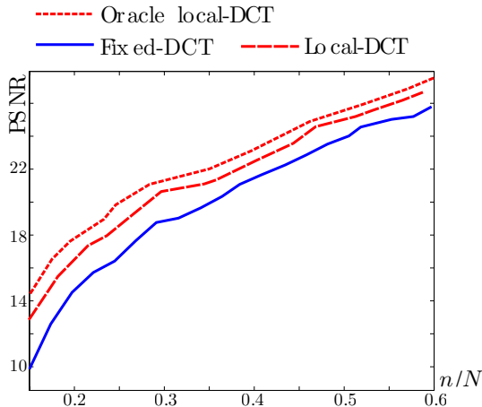
Fig. 5. Recovery results for the signal of figure 4 for various rate of sensing n/N , in the noiseless setting y = \Phi f .
