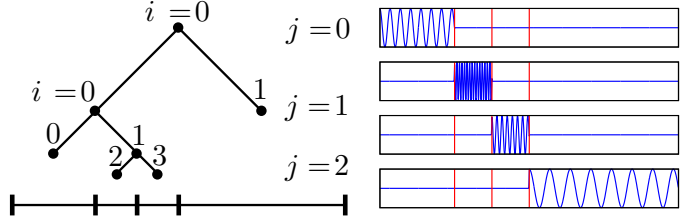
Fig. 2. A dyadic tree \lambda defining a spatial segmentation (left) ; some local cosine basis functions \psi_{i,s}^j of the basis \mathcal{B}(\lambda) (right).
