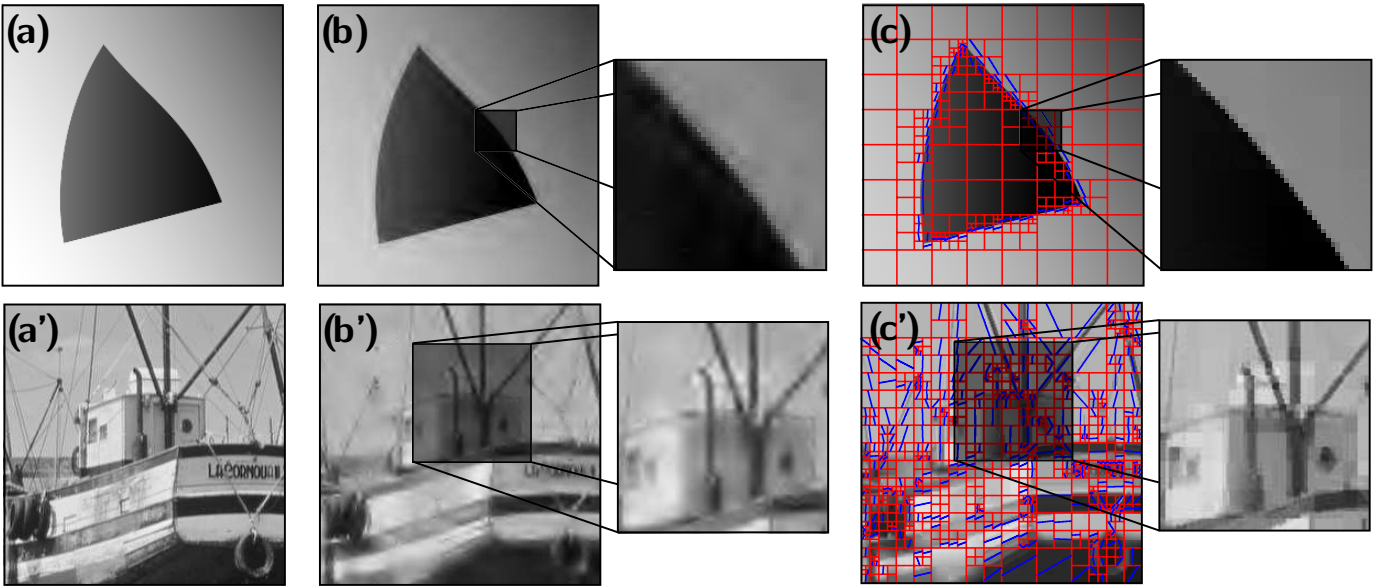
Fig. 11. (a,a') original image ; (b) compressive sensing reconstruction using the translation invariant wavelet frame, n = N/6 (PSNR=37.1dB) ; (c) reconstruction using iteration in a best bandlet basis (PSNR=39.3dB). (b') wavelet frame, PSNR=22.1dB, (c') bandlet basis, PSNR=23.9dB.
