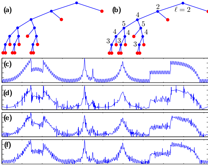
Fig. 6. (c) original signal, N = 4096 ; (d) recovery using orthogonal wavelets, n = N/3 (PSNR=23.77dB); (e) recovery using best wavelet packets basis, n = N/3 (PSNR=26.50dB), the corresponding dictionary tree is shown in (a); (f) recovery using best non-stationary wavelet packets basis, n = N/3 (PSNR=29.42dB), the corresponding dictionary tree is shown in (b).
