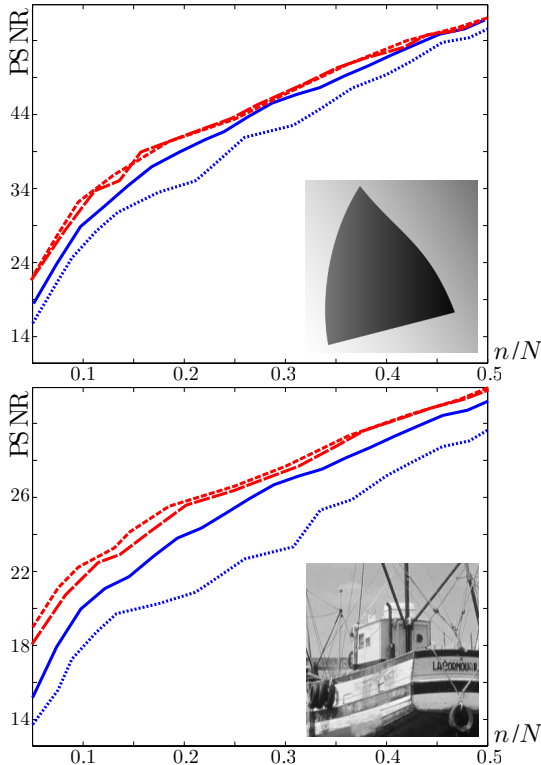
Fig. 10. Recovery results for various rate of sensing n/N , in the noiseless setting y = \Phi f .
