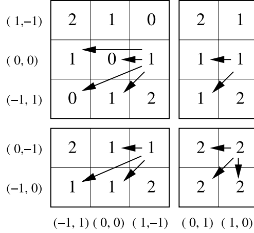
FIGURE 3. Examples of non trivial cases
