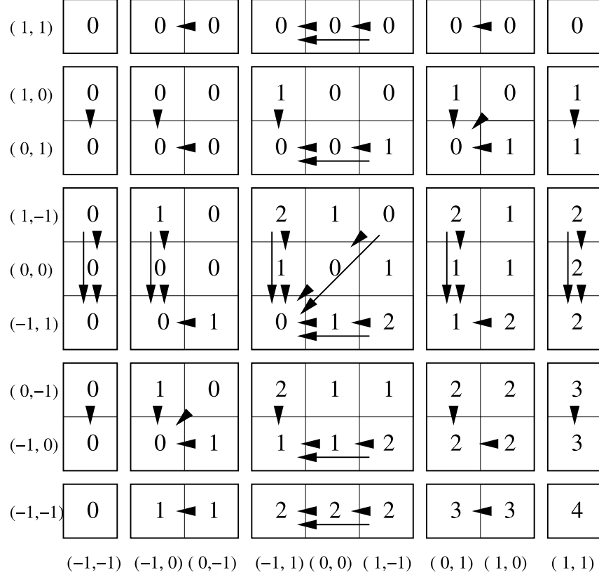
FIGURE 2. The coupling rates between two sites for the two species model. Possible coupled jumps, represented by arrows, are subject to three restrictions: arrows connect two cells in the same sub-array, point leftwards and/or downwards, cannot point to a larger value than the initial one. All trivial arrows have been represented, leaving four non trivial cases.
