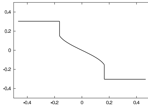
FIGURE 1. Starting from an initial condition u_0(x) = \lambda(\mathbf{1}_{\{x < 0\}} - \mathbf{1}_{\{x \geq 0\}}) , the hydrodynamic limit may develop two shocks going in opposite directions at constant speeds and a rarefaction fan in-between. Here c = .145 and \lambda = .303 .
