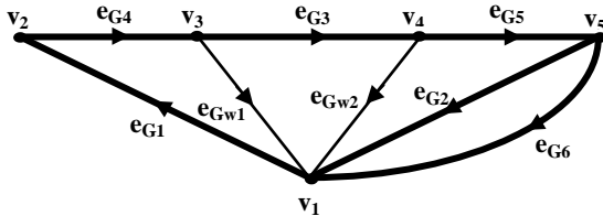
Fig. 2. dynamic network graph G_w of the Cuk converter
