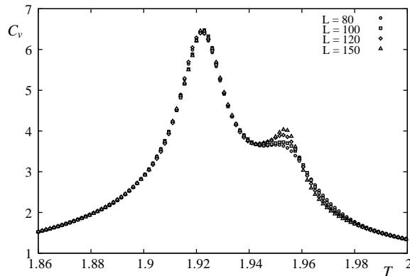
FIG. 8: Specific heat are shown for various sizes L as a function of temperature.
