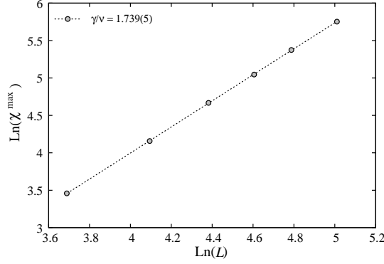
FIG. 12: Maximum sublattice susceptibility \chi^{\max} versus L in the \ln - \ln scale. The slope of this straight line gives \gamma/\nu .
