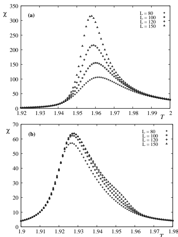
FIG. 9: Susceptibilities of sublattice 1 (a) and 3 (b) are shown for various sizes L as a function of temperature.
