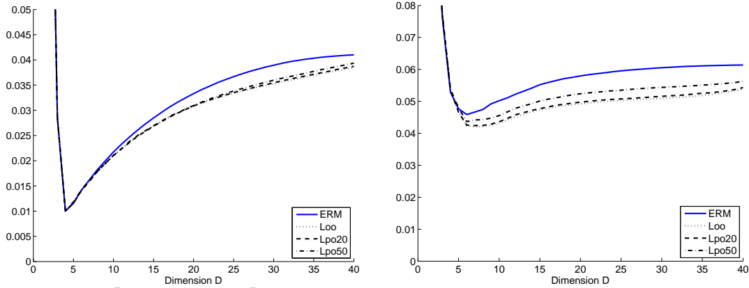
Figure 3: \mathbb{E} \left[ \left\| s - \widehat{s}_{\widehat{m}_{\mathfrak{F}}(D)} \right\|_n^2 \right] as a function of D for \mathfrak{F} among ‘ERM’ (empirical risk minimization), ‘Loo’ (Leave-one-out), ‘Lpo(20)’ (Lpo p with p = 20 ) and ‘Lpo(50)’ (Lpo p with p = 50 ). Left: homoscedastic ( s_2, \sigma_c ). Right: heteroscedastic ( s_3, \sigma_{pc,3} ). All curves have been estimated from N = 10\,000 independent samples; error bars are all negligible in front of visible differences (the larger ones are smaller than 8 \cdot 10^{-5} on the left, and smaller than 2 \cdot 10^{-4} on the right). The curves D \mapsto \left\| s - \widehat{s}_{\widehat{m}_{\mathfrak{F}}(D)} \right\|_n^2 behave similarly to their expectations.
