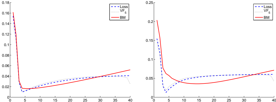
Figure 4: Comparison of the expectations of \|s - \widehat{s}_{\widehat{m}(D)}\|_n^2 (‘Loss’), \text{crit}_{\text{VF}_V}(D) (‘VF 5 ’) and \text{crit}_{\text{BM}}(D) (‘BM’). Data are generated as explained in Section 3.3.1. Left: homoscedastic ( s_2, \sigma_c ). Right: heteroscedastic ( s_2, \sigma_{pc,3} ). Expectations have been estimated from N = 10\,000 independent samples; error bars are all negligible in front of visible differences (the larger ones are smaller than 5 \cdot 10^{-4} on the left, and smaller than 2 \cdot 10^{-3} on the right). Similar behaviours are observed for every single sample, with slightly larger fluctuations for \text{crit}_{\text{VF}_V}(D) than for \text{crit}_{\text{BM}}(D) . The curves ‘BM’ and ‘VF 5 ’ have been shifted in order to make comparison with ‘Loss’ easier, without changing the location of the minimum.
