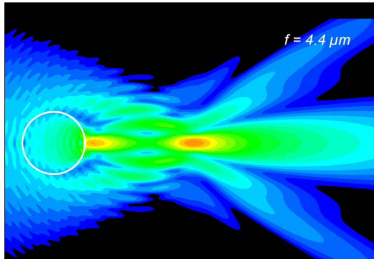
Fig. 4. (2000KB) Movie of the electric field intensity map for d decreasing from d = 7 \mu\text{m} to d = 0 \mu\text{m} and N.A. \approx 1 . The white circle represents the sphere cross-section.
