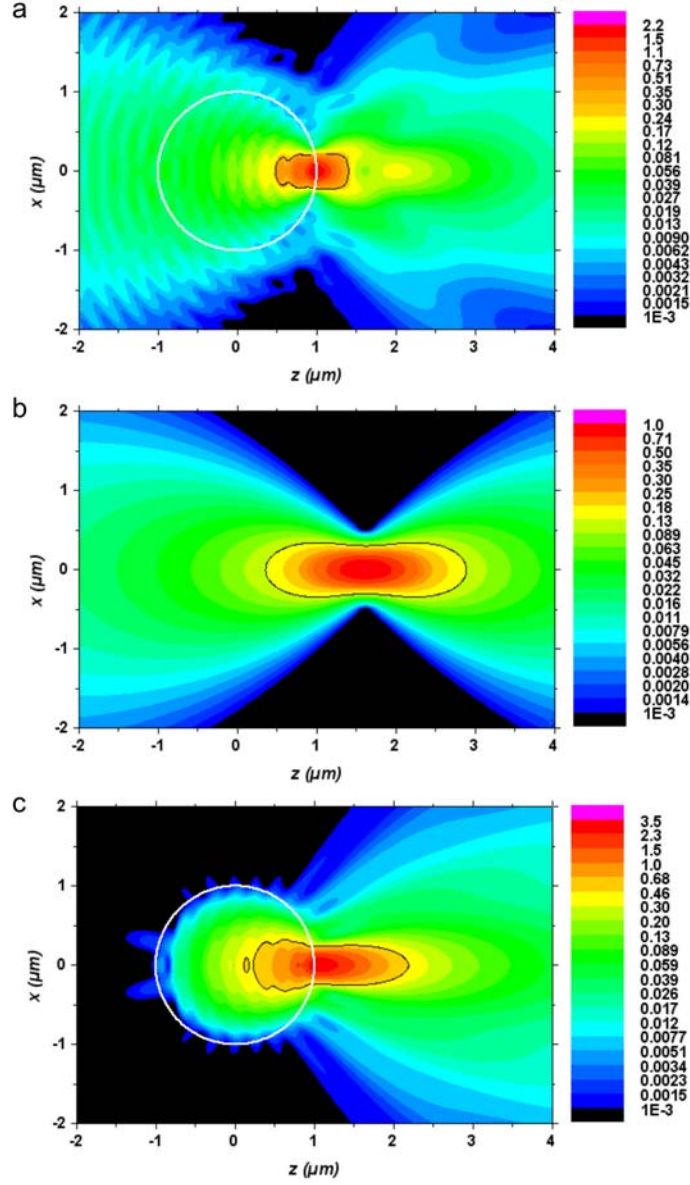
Fig. 1. (a) Total electric field intensity map for d = 1.62 \mu\text{m} . The white circle represents the microsphere section, the thin black line represents the I_{max}/e^2 intensity contour. (b) and (c) display the intensity maps of the incident and scattered fields. The coherent summation of these two fields leads to the total intensity presented in (a).
