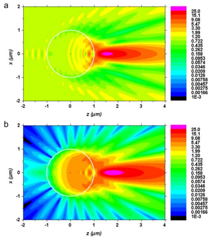
Fig. 2. Electric field intensity maps of (a) the scattered field and (b) the total field in the same conditions than previously but the sphere is illuminated by a plane wave. The incident intensity is normalized to be unitary per surface unit.
