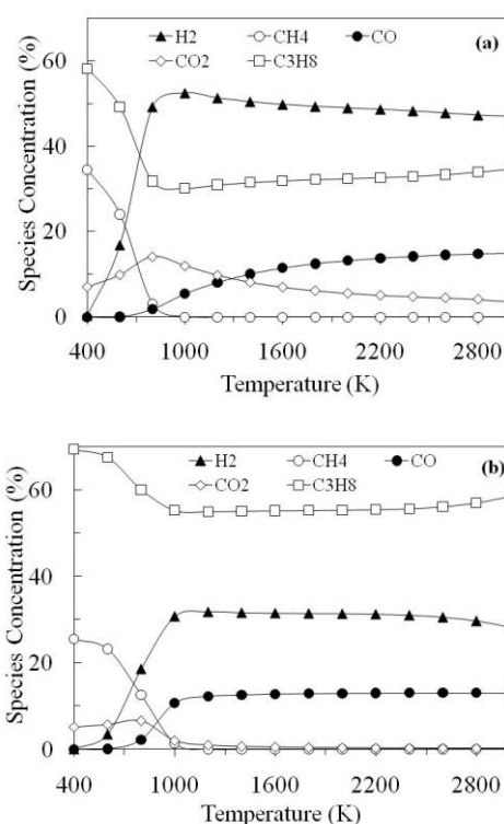
Figure 10: Computed species concentration at thermodynamic equilibrium as a function of temperature for different H_2O-C_3H_8 systems at total flow rate and \gamma -factor of about 80 L/min and 50%, respectively: (a) H_2O/C_3H_8 = 19 and (b) H_2O/C_3H_8 = 4 .
