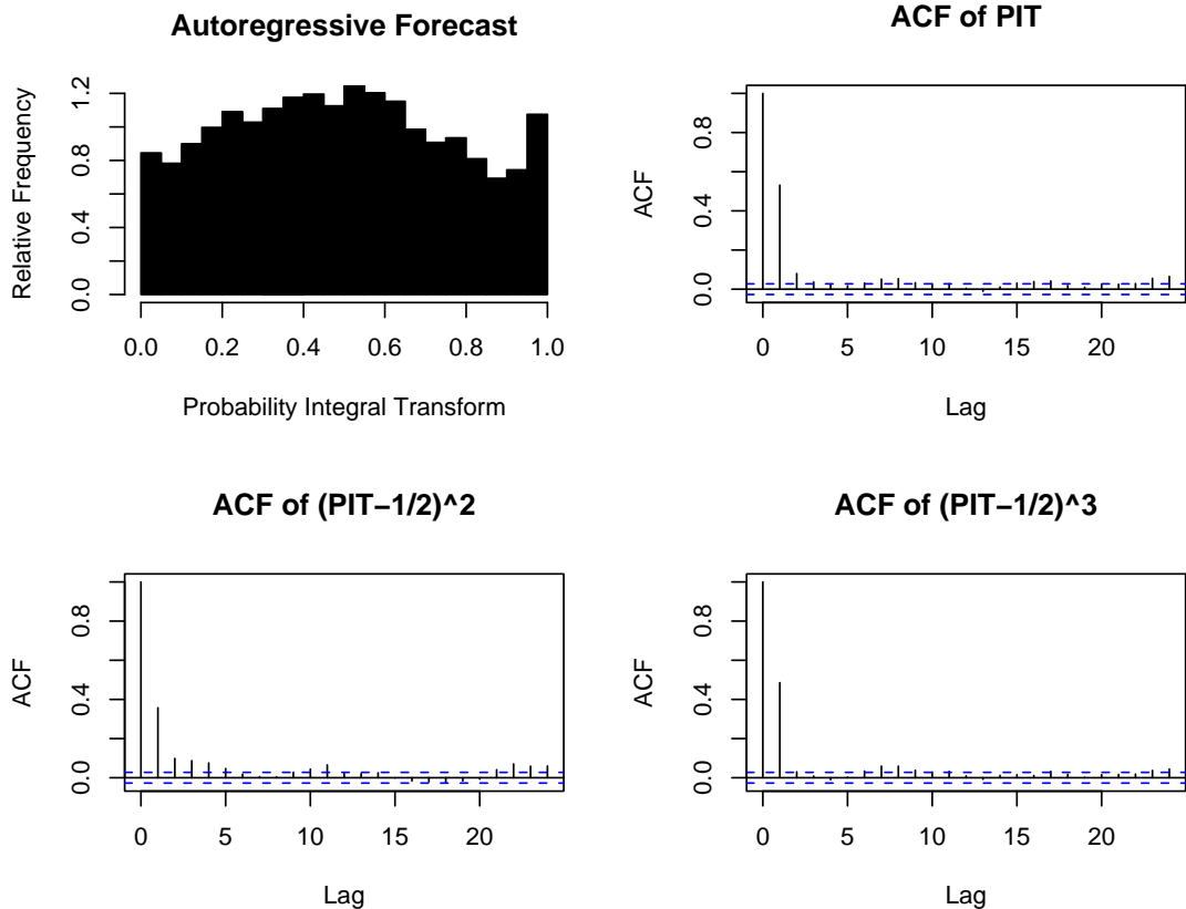
Figure 5: Same as Figure 4, but for autoregressive forecasts.
