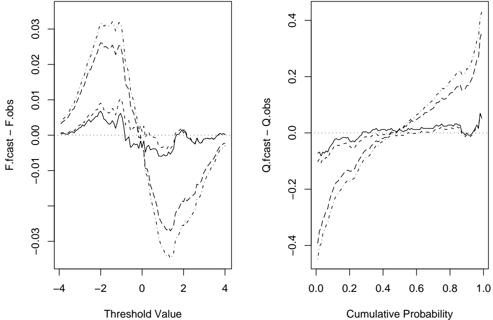
Figure 2: Marginal calibration plot for the ideal forecaster (solid line), climatological forecaster (short dashes), unfocused forecaster (dot-dashed line) and Hamill’s forecaster (long dashes). The presentation is in terms of CDFs (left) and in terms of quantiles (right), respectively.
