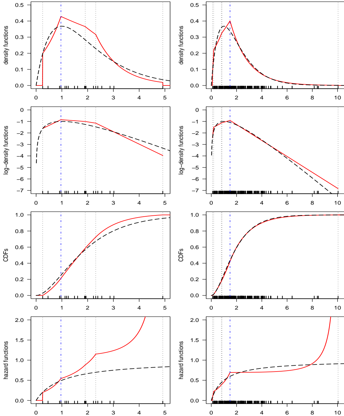
FIG 1. Examples for log-concave density, log-density, CDF, and hazard rate estimation for n = 20, 200 (--- true functions, - estimators). The dotted vertical lines indicate the set \hat{S}_n(\hat{\varphi}_n) . The ·-·- vertical lines are placed at the mode of the estimated density.
