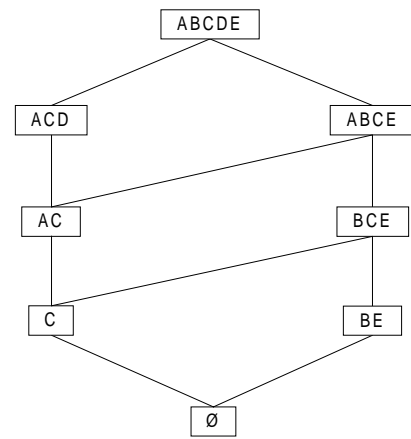
Figure 2. Closed itemset lattice
