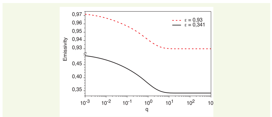
Figure 2 Emissivity variation (as calculated using Sayapina's model) for a \theta = 15^\circ observation direction vs. roughness parameter q
