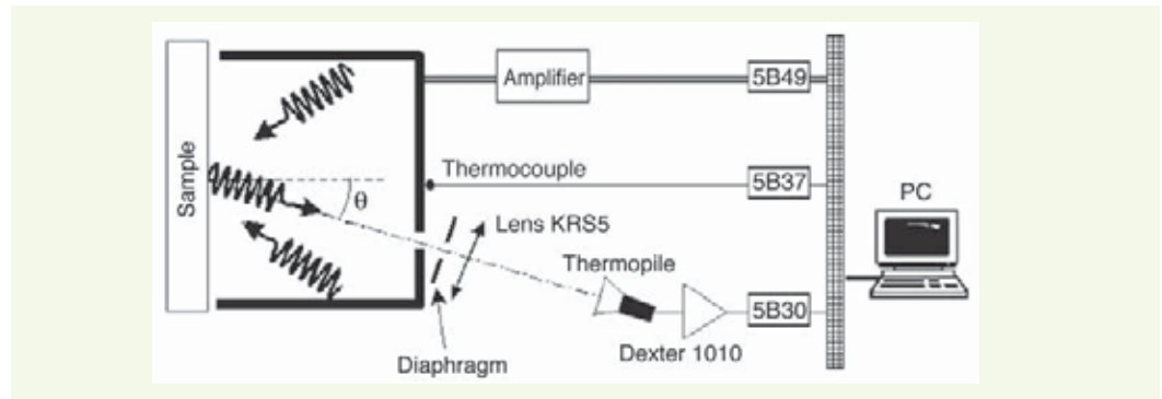
Figure 1 Simplified diagram of the portable emissometer
