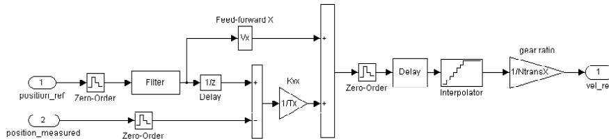
Figure 7: Position Controller
