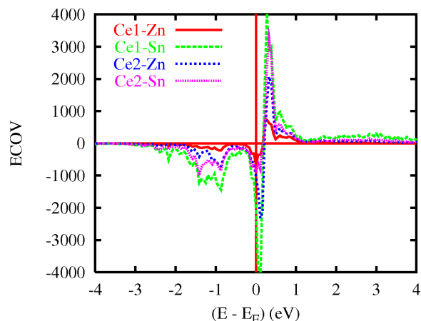
Fig. 3 (color online). Non-magnetic CeZnSn: chemical bonding based on the ECOV criterion ( cf. text). Zero energy is with respect to the Fermi level E_F .
