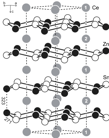
Fig. 1. The crystal structure of CeZnSn. Cerium, zinc, and tin atoms are drawn as light grey, black filled, and open circles, respectively. The puckered Zn_3Sn_3 hexagons, relevant interatomic distances, and the crystallographically independent cerium sites are indicated.
