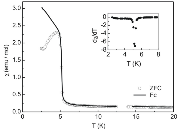
Fig. 7. Low-temperature susceptibility (zero-field-cooling and field-cooling modus) of CeZnSn at 100 Oe (kink-point measurement). The inset shows the derivative d\chi/dT of the zero-field-cooling curve with a sharp peak at the Curie temperature of T_C = 5.2 K.
