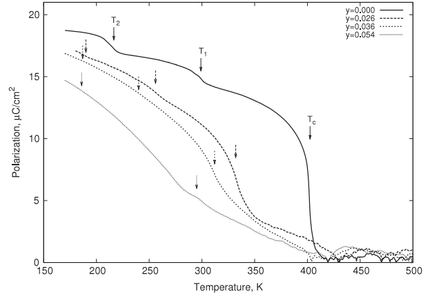
Figure 5. Root mean square polarization of \text{Ba}_{1-y}\text{La}_y\text{Ti}_{1-y/4}\text{O}_3 compounds.
