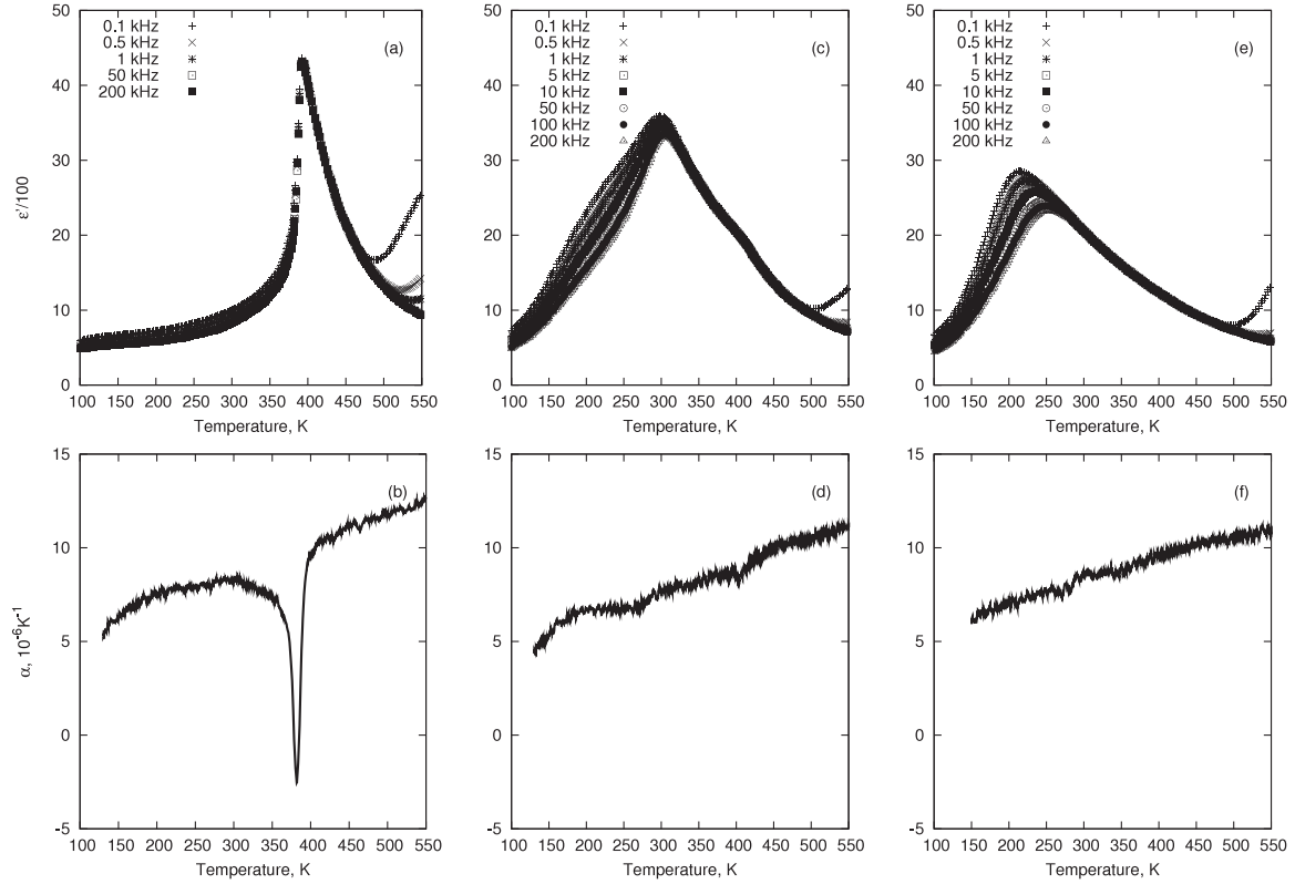
Figure 6. Temperature dependence of the real part of the permittivity \varepsilon' ((a), (c), (e)), and the thermal expansion coefficient \alpha ((b), (d), (f)) for ceramics with composition \text{Ba}_{0.90}\text{Bi}_{0.067}\text{Ti}_{1-x}\text{Zr}_x\text{O}_3 : (a), (b) x = 0.0 ; (c), (d) x = 0.05 ; (e), (f) x = 0.1 .
