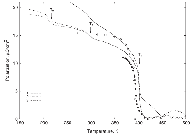
Figure 2. Polarization as a function of temperature for \text{BaTiO}_3 obtained by method A (1), method B (2) and method C (3): O, data from [19]; ●, data from [20].
