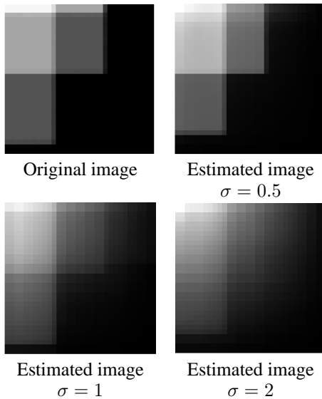
Figure 3: The original image (left panel) and the EWA estimated image from noisy observations with \sigma = 0.5 , \sigma = 1 and \sigma = 2 , respectively. In all cases n = 200 and k = 15 .
