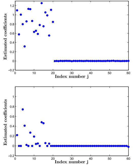
Figure 2: A typical result of the EWA (top panel) and the Lasso (bottom panel) in the setup of Example 1 with n = 200 , M = 500 and S = 20 . For better visibility, only 60 first coefficients are plotted.
