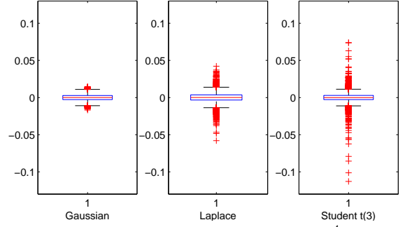
Figure 1: The boxplots of a sample of size 10^4 drawn from the scaled Gaussian (left panel), Laplace (central panel) and Student t(3) (right panel) distributions. In all three cases the location parameter is 0 and the scale parameter is 10^{-2} .
