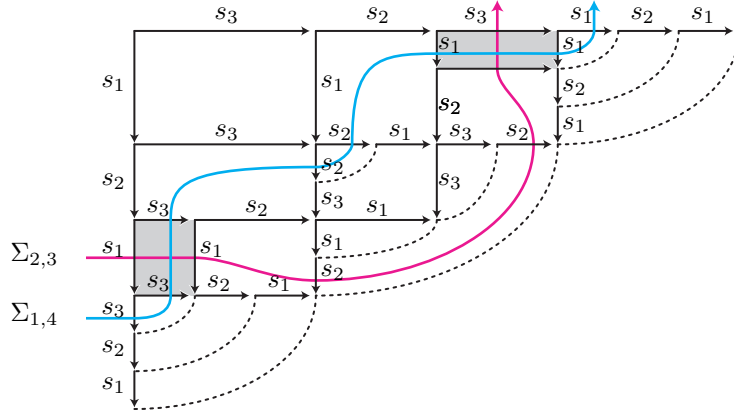
FIGURE 4. Reversing diagram for \bar{s}_1\bar{s}_2\bar{s}_3\bar{s}_1\bar{s}_2\bar{s}_1s_3s_2s_3s_1s_2s_1 . There are eight nontrivial tiles (four type I hexagons and four type II squares), giving \text{compl}_{\curvearrowright}(s_1s_2s_1s_3s_2s_1, s_3s_2s_3s_1s_2s_1) = 8 . Collapsing the \epsilon -edges in the above diagram yields the bottom van Kampen diagram of Figure 2. The failure of optimality is witnessed by the two intersections of the separatrices \Sigma_{1,4} and \Sigma_{2,3} .
