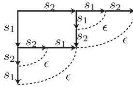
FIGURE 3. Reversing diagram associated with the sequence (*) , i.e., the reversing diagram of the pair (s_1s_2s_1, s_2s_1s_2) . Metric aspects are ignored, so the reversing diagram is always considered up to a piecewise affine deformation.
