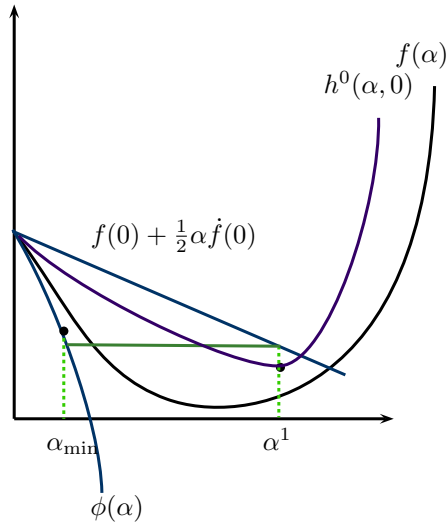
Figure 4: Minorizing \alpha^j in the convex case : Illustration of inequality (3.26)
