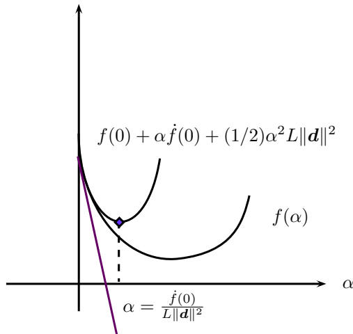
Figure 1: Constant stepsize idea from [1]
