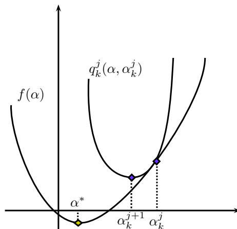
Figure 2: MM quadratic line search in the convex case
