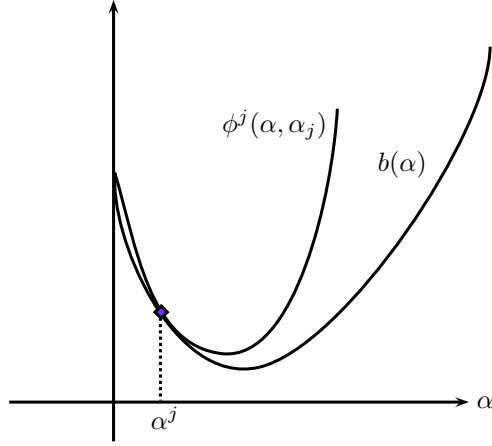
Figure 6: The construction of the tangent majorant of b(\alpha) at \alpha^j
