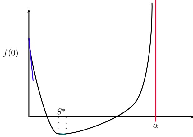
Figure 3: The function f(\alpha) in the convex case and \bar{\alpha} \neq \infty . S^* is the set of stationary points of f .
