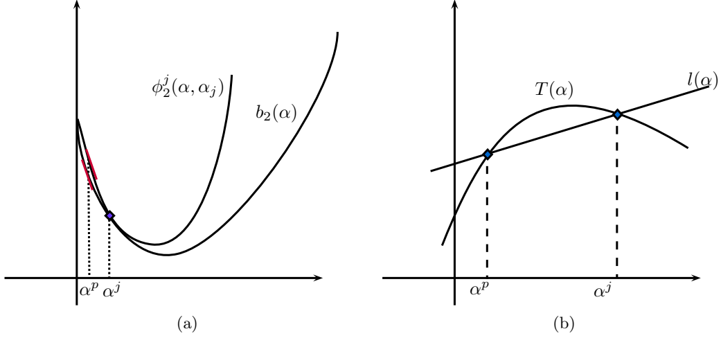
Figure 5: Construction of the tangent majorant
