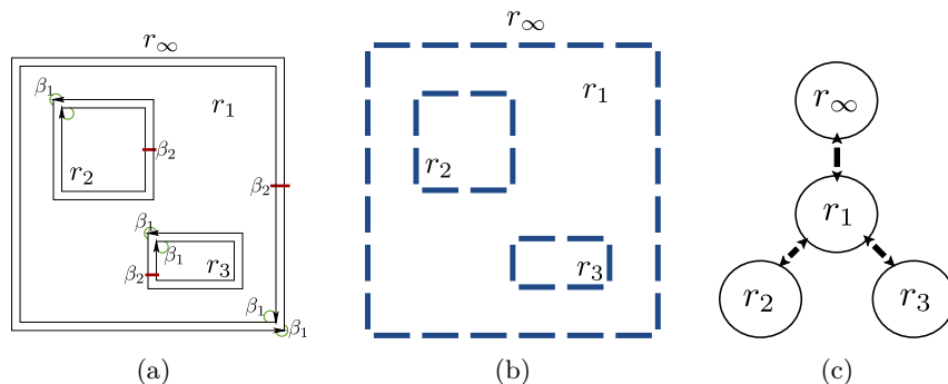
Figure 3: The three different models composing a topological map. (a) A 2-map representing the topology with darts and \beta_i relationships; (b) A geometrical matrix that points out active lines and pointels; corresponding elements are linked together (for visibility reasons, dotted lines represent only up/down relations between regions); (c) A tree of regions for inclusion relations.
