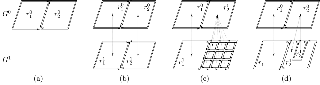
Figure 5: Main steps of the construction process of a top-down pyramid. (a) Initial step: the pyramid is composed of a single level G^0 ; (b) Duplicate and link: G^1 is a copy of G^0 and corresponding elements are linked together (for visibility reasons, dotted lines represent only up/down relations between regions); (c) Split: r_2^0 is split into a set of square-unit regions enclosing a single pixel; (d) Merge and simplify: some of the created regions are merged and draw r_2^1 and r_3^1 .
