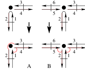
Figure 8: 1-sewing operations when processing dangling edge (1,2). (A) One perpendicular edge: 1-sew (1,4) and (3,2). (B) Two perpendicular edges: 1-sew (1,4) and (5,2).
