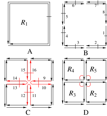
Figure 6: Decomposition in 4 steps of the splitting process applied on a region R_1 enclosing 4 pixels. (A) Initial region. (B) Splitting edges: darts 1 to 8 are stored into list (external border of R_1 ). (C) Insertion of 4 dangling edges while testing darts 1, 3, 5 and 7. (D) Sewing correctly dangling edges while testing darts 9 and 13.
