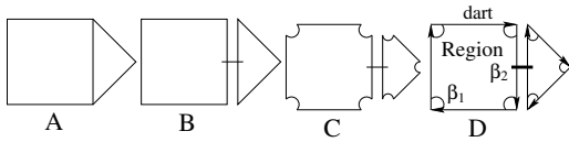
Figure 1: Construction of a 2-map by successive decompositions. (A) Original image. (B) Disconnected faces. (C) Disconnected edges. (D) 2-map: darts are the basic elements represented by arrows, \beta_1 relations are represented with arcs and \beta_2 with bold segments.
