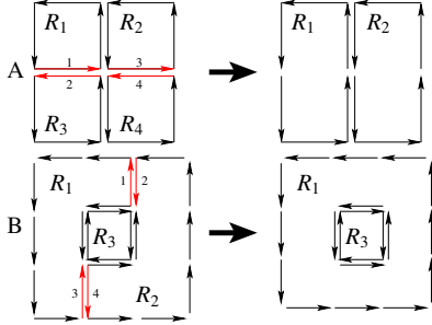
Figure 9: Configurations encountered during the merging operation between two adjacent regions. (A) Simple adjacency between (R_1, R_3) and (R_2, R_4) : the corresponding edges (1,2) and (3,4) are removed if the merging criterion is verified. (B) Multi-adjacency between (R_1, R_2) : if (1,2) has been removed, (3,4) is removed independently of the merging criterion.
