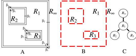
Figure 3: The three different models composing a topological map. (A) A 2-map representing the topology with darts and \beta_i relations. (B) A geometrical matrix that points out active lines and pointlets. (C) A tree of regions for inclusion relations.
