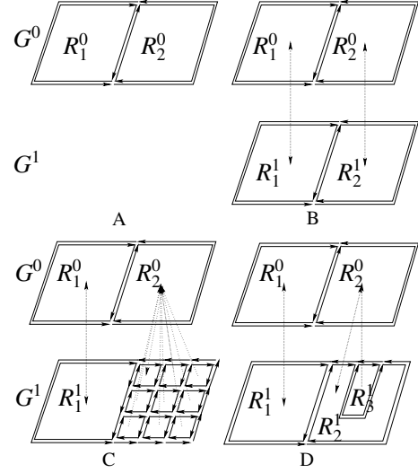
Figure 5: Main steps of the construction process of a top-down pyramid. (A) Initial step: the pyramid is composed of a single level G^0 . (B) Duplicate and link: G^1 is a copy of G^0 and corresponding elements are linked together (for visibility reasons, dotted lines represent only up/down relations between regions). (C) Split: R_2^0 is split into a set of square-unit regions enclosing a single pixel. (D) Merge and simplify: some of the created regions are merged and draw R_2^1 and R_3^1 .
