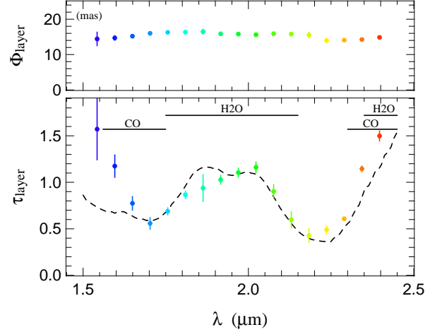
Fig. 5. Size and optical depth of the layer surrounding the photosphere, as extracted by a fit of the visibility curves (Sec. 4). The dashed curve is a fit with \text{H}_2\text{O} and \text{CO} opacities assuming T_l = 1800 \text{ K} (T. Verhoelst, private communication). A continuum opacity of \tau \approx 0.2 was added.
