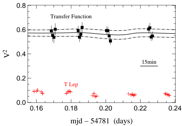
Fig. 1. Example of observation sequence, on the baseline G0-H0 and for the spectral bin 1.59 \mu\text{m} . The interpolated TF is represented.
