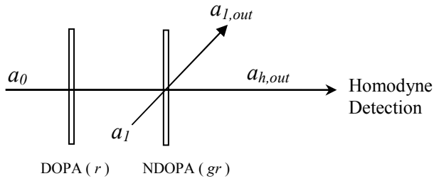
FIG. 2: Equivalent model for the Bogoliubov transform U : a perfect single-mode degenerate optical parametric amplifier (DOPA) with squeezing parameter r is followed by a perfect non-degenerate optical parametric amplifier (NDOPA) with squeezing parameter gr .
