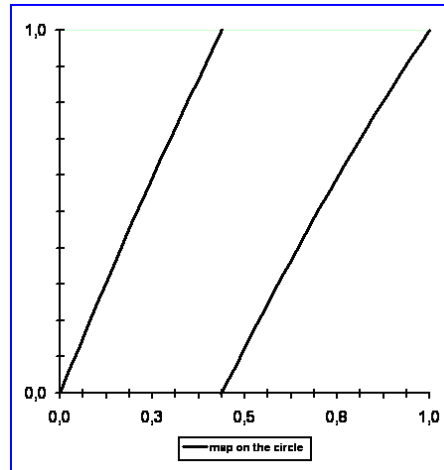
Figure 1: Graph of the map f(x) = 2x + 0.5x(1 - x)
