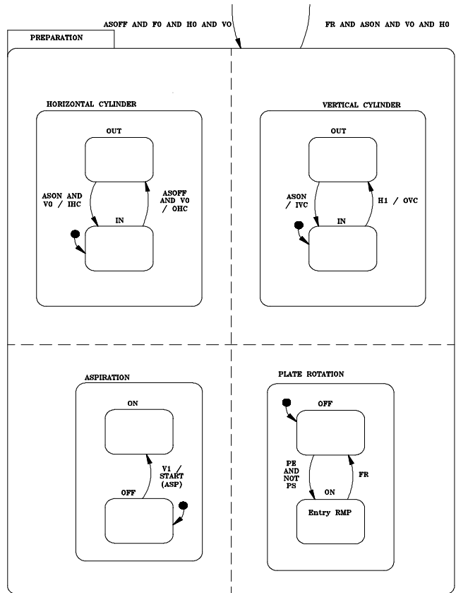
Figure 8) "Preparation" state included in "Automatic" state
