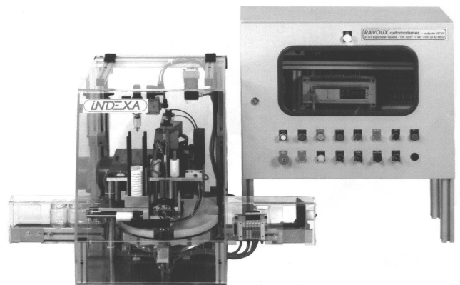
Figure 2) INDEXA machine
